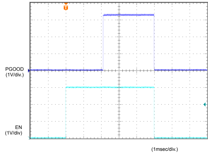
Figure 14. PGOOD Delay (Start up-Shut down)
