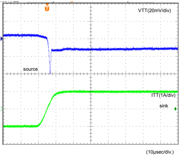
Figure 9. DDR1 (-1A to +1A)
