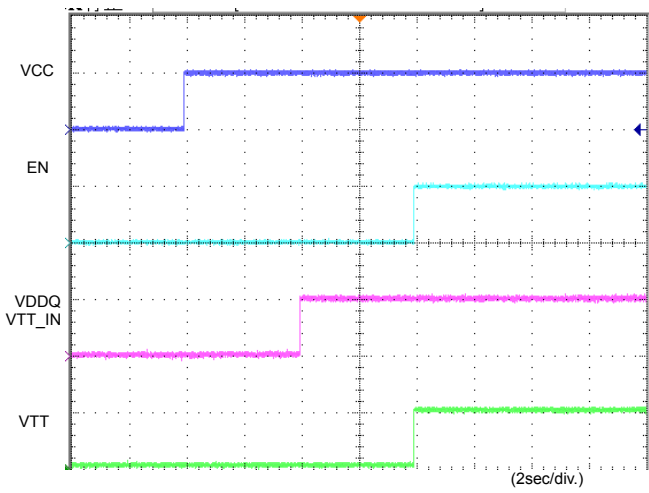
Figure 11. Input Sequence2
