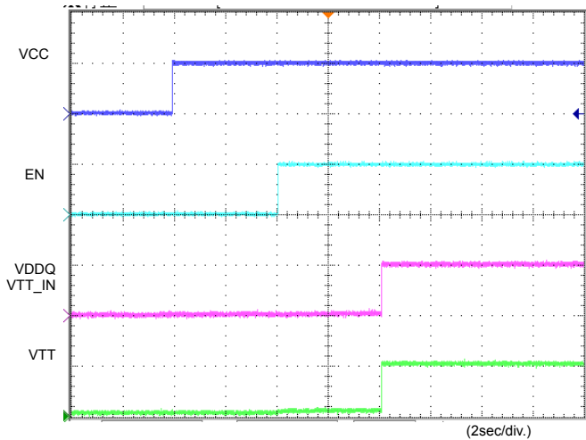
Figure 10. Input Sequence1
