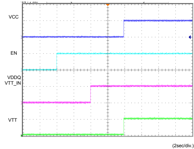
Figure 12. Input Sequence3
