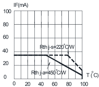
FIG.3 Green MAXIMUM FORWARD DC CURRENT VS AMBIENT TEMPERATURE ( T_{jmax}=110^{\circ}\text{C} )
