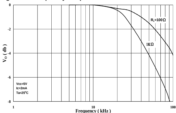
Figure 17. Frequency Response
