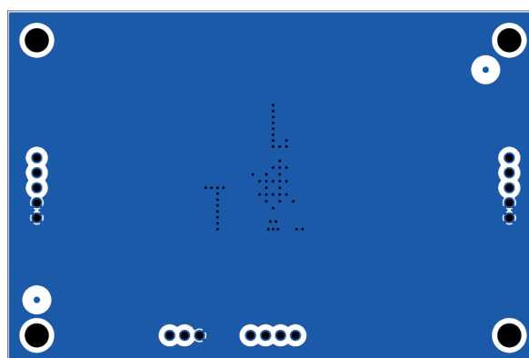
Bottom (GND)
