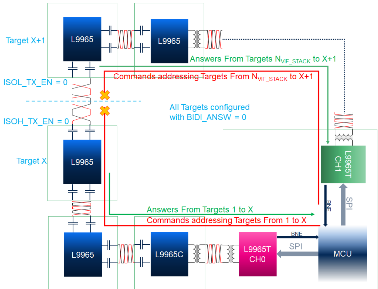
Figure 21. Double data rate using dual access commands
