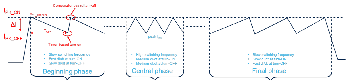
Figure 29. Pre-charge current waveform
