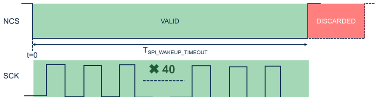
Figure 22. Wakeup condition by SPI Target
