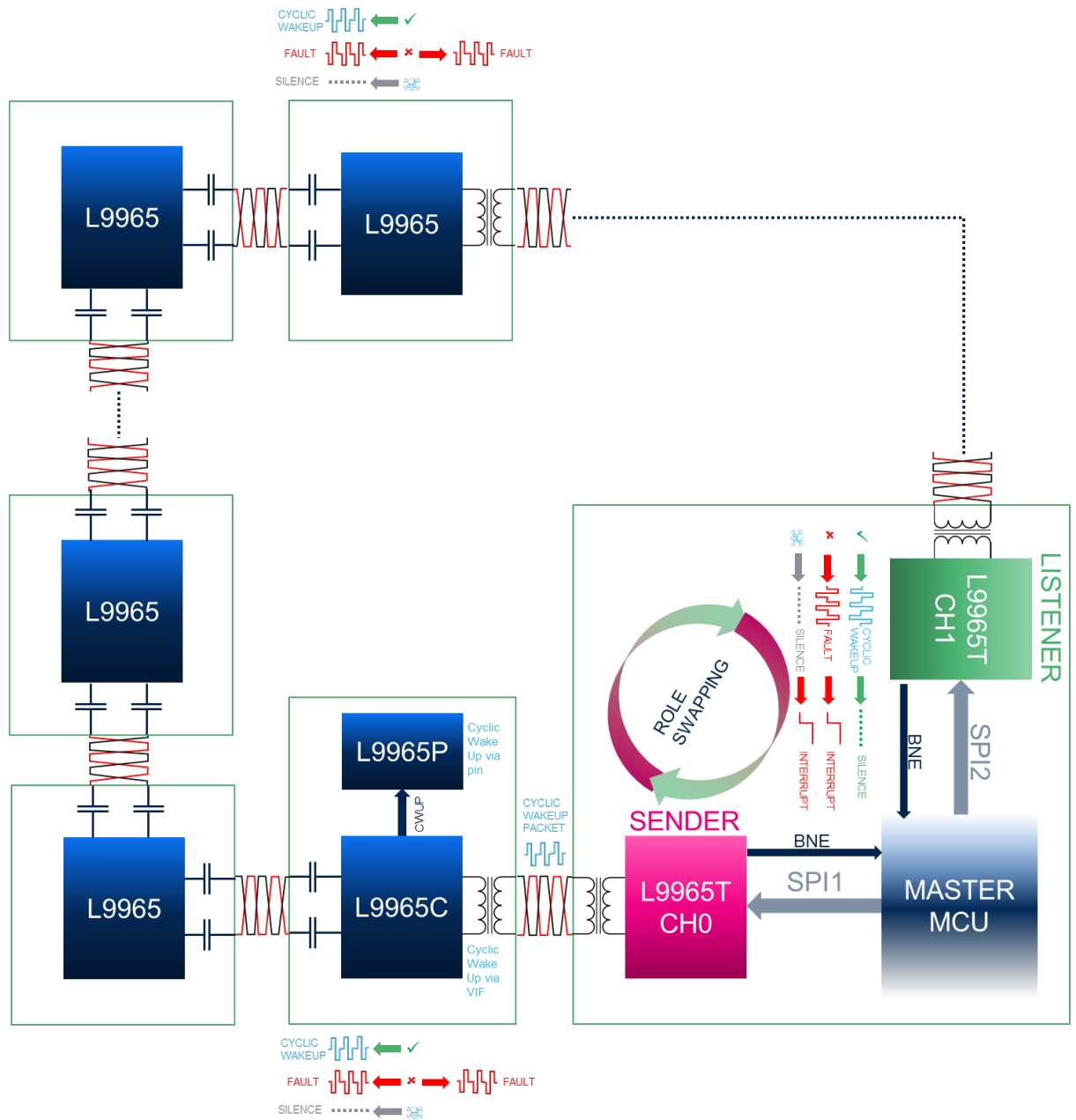
Figure 25. Cyclic wakeup operation
