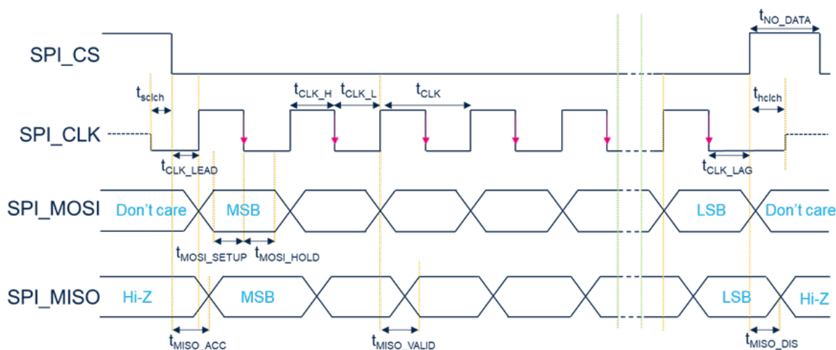
Figure 18. SPI Target timing diagram
