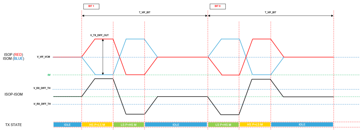
Figure 19. VIF Waveform
