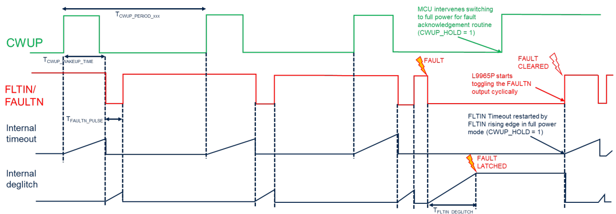
Figure 12. FLTIN integrity check in low power mode (example of fault detected by L9965P/L99BM2P)
