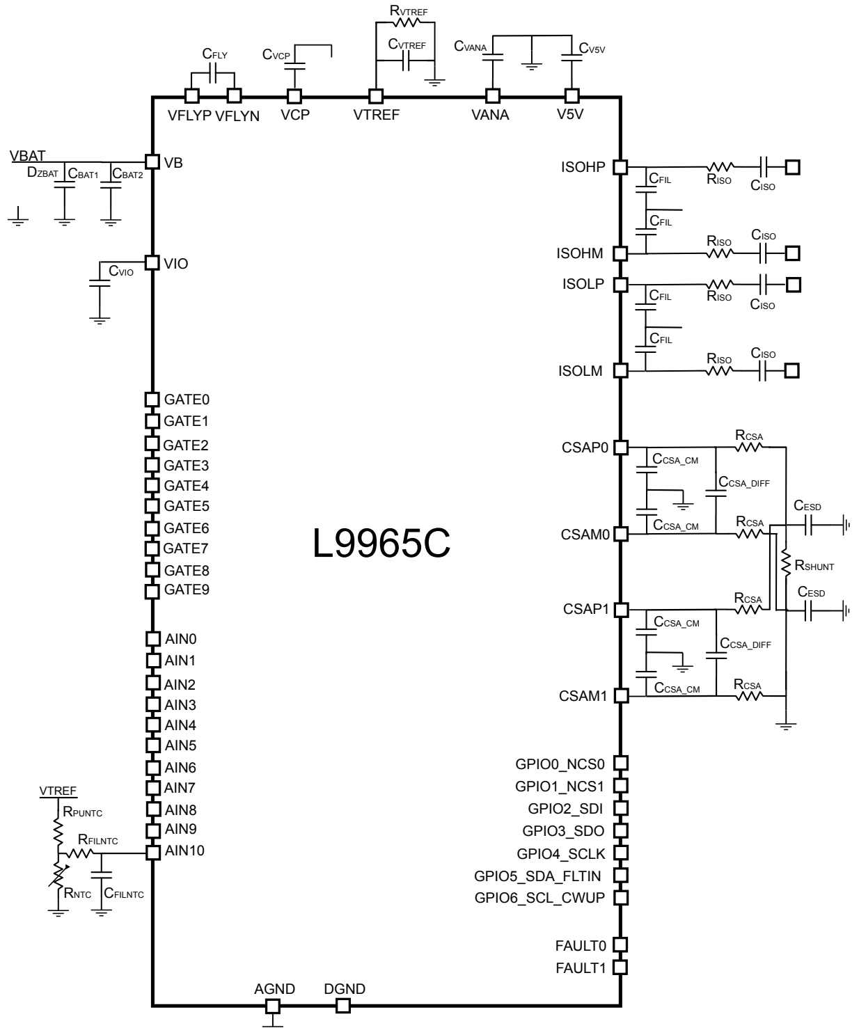
Figure 30. Typical application circuit
