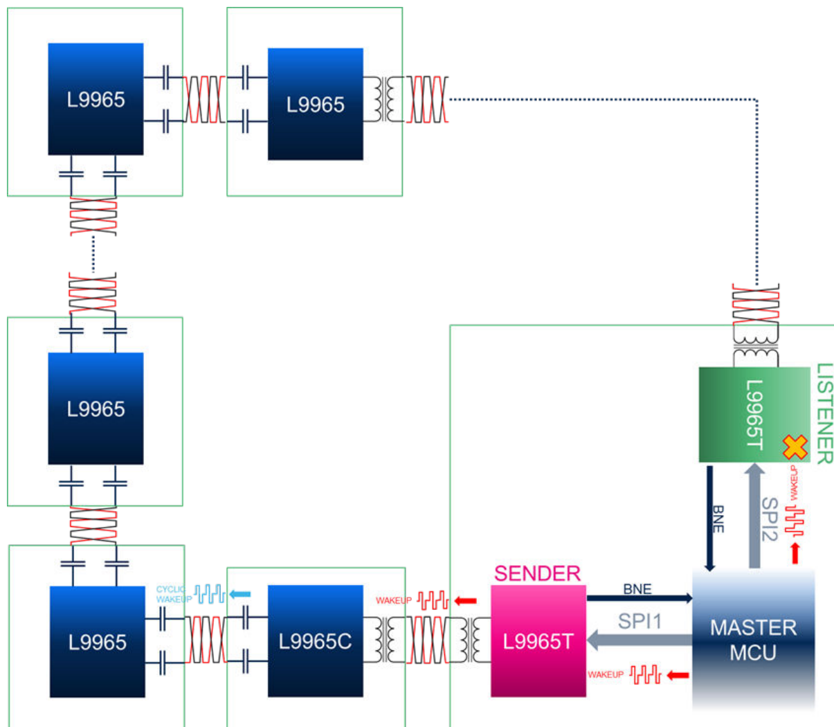
Figure 23. Wakeup by MCU
