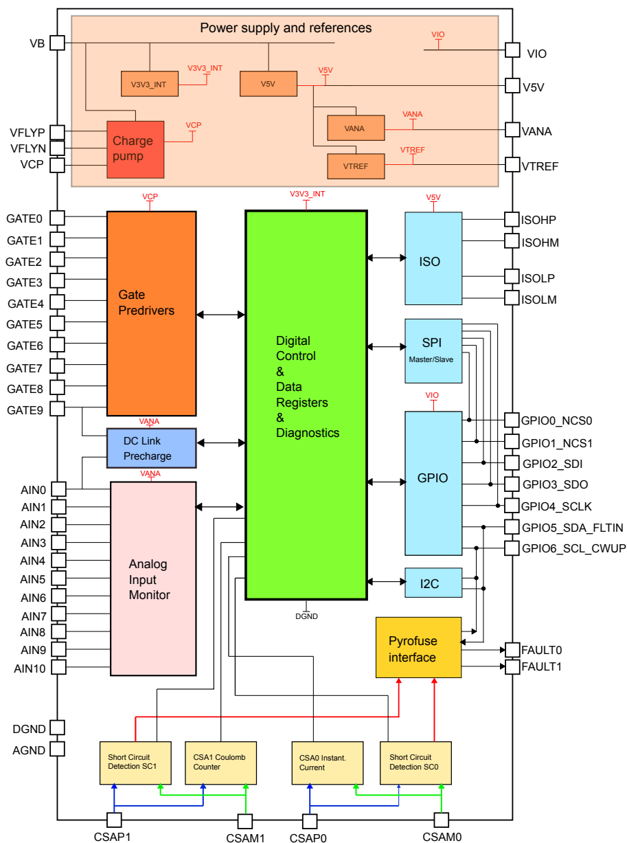
Figure 2. L9965C Block diagram
