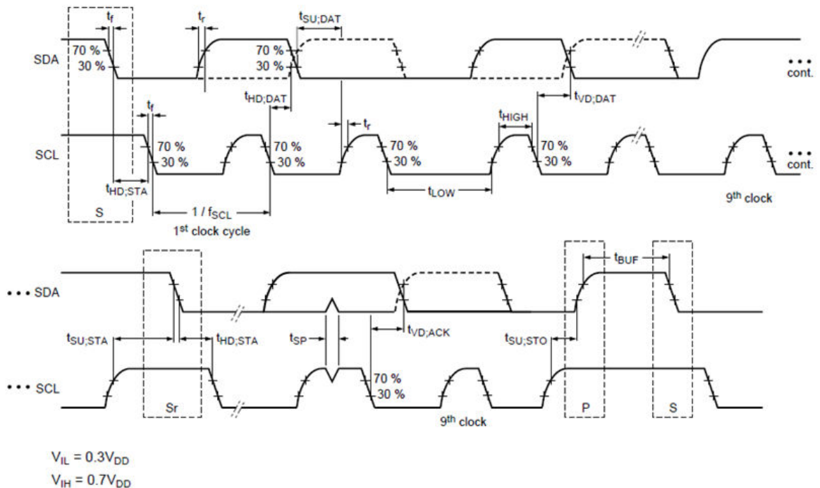
Figure 27. I2C Controller timing
