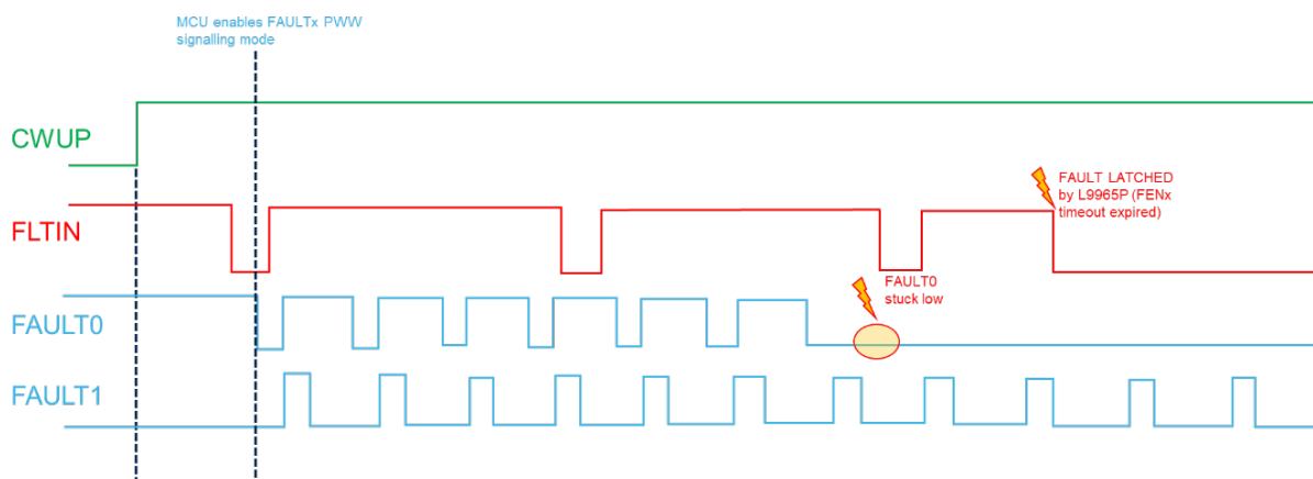
Figure 17. FAULTx lines integrity check in PWM mode
