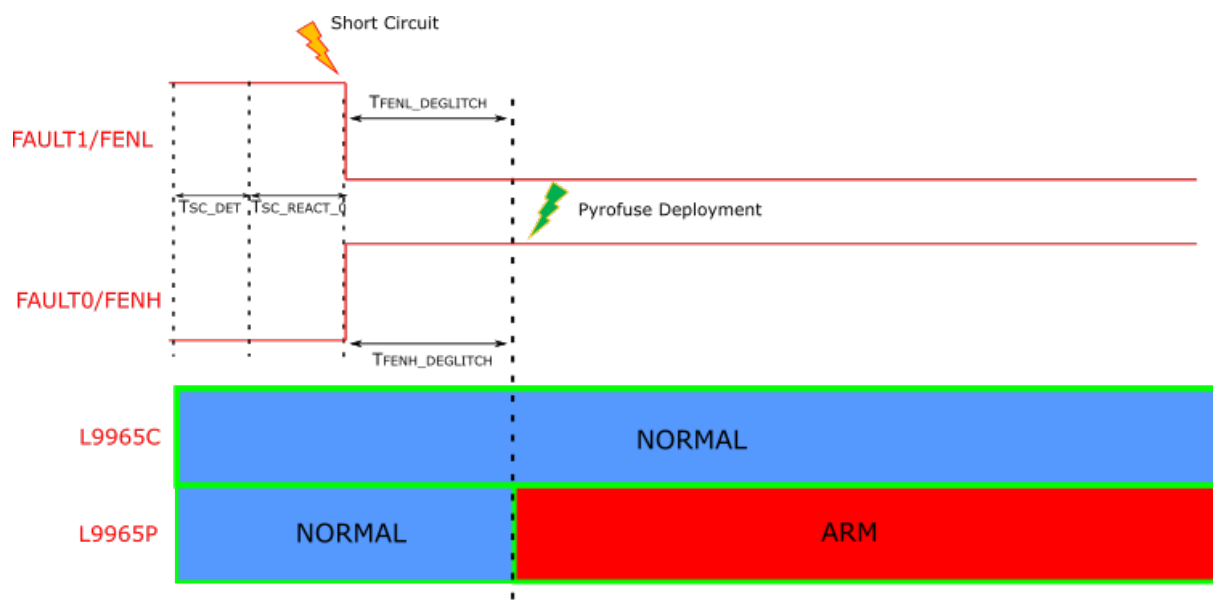
Figure 14. Pyro-Fuse deployment when L9965C is in NORMAL and L9965P/L99BM2P is in WAKEUP state
