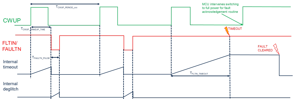
Figure 11. FLTIN integrity check in low power mode (example of timeout detected by L9965C)
