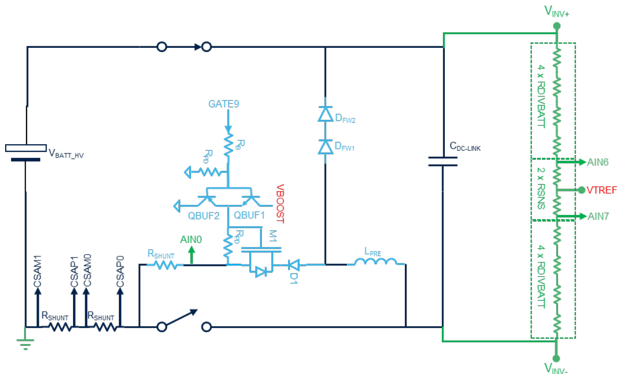
Figure 28. DC-Link precharge controller reference design
