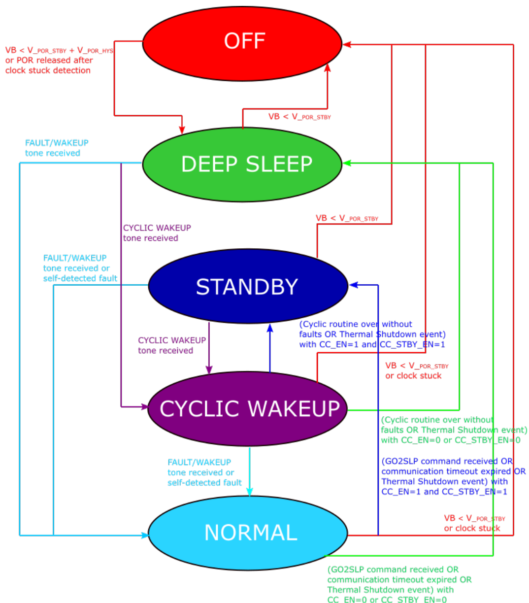
Figure 5. Device functional states
