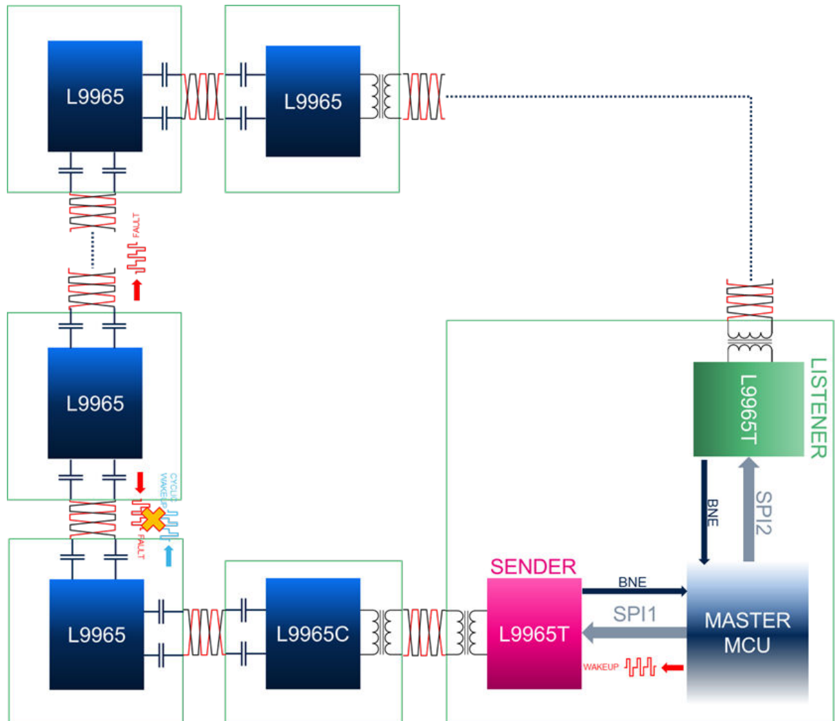
Figure 24. Wakeup by Fault
