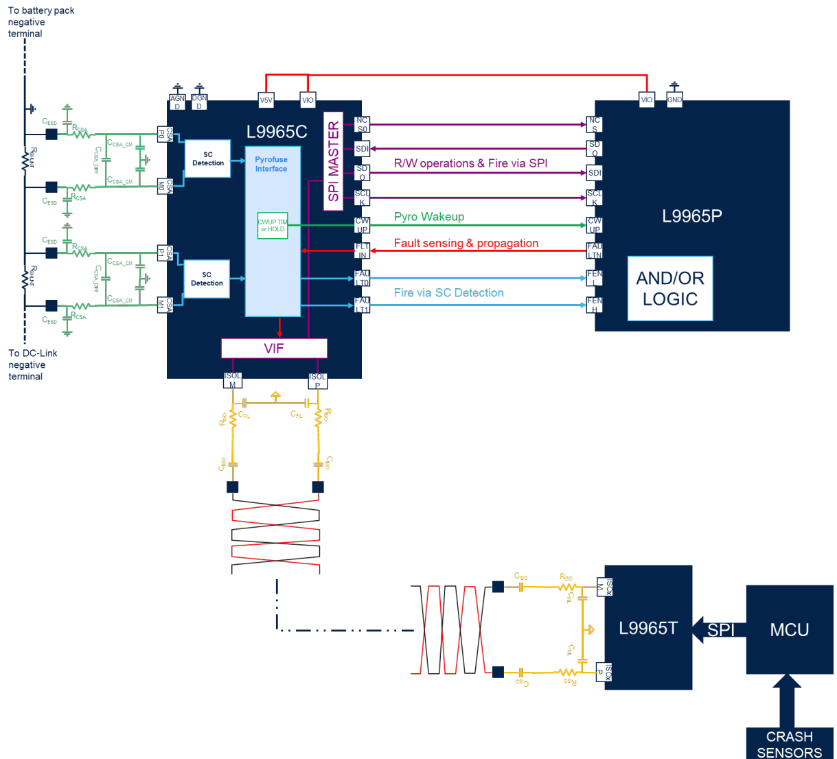
Figure 9. Interfacing L9965C to L9965P/L99BM2P
