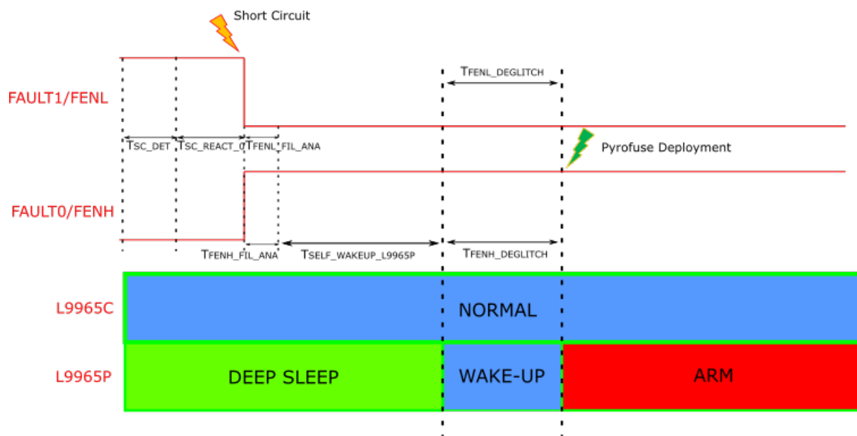
Figure 13. Pyro-Fuse deployment when both L9965C is in NORMAL and L9965P/L99BM2P is in DEEP SLEEP state
