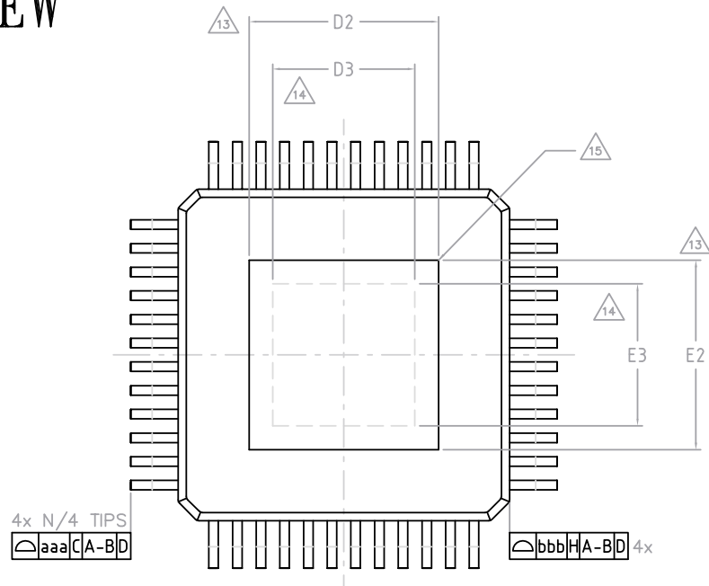
Figure 31. TQFP48L (7x7x1 mm exposed pad down) package outline - top and bottom
