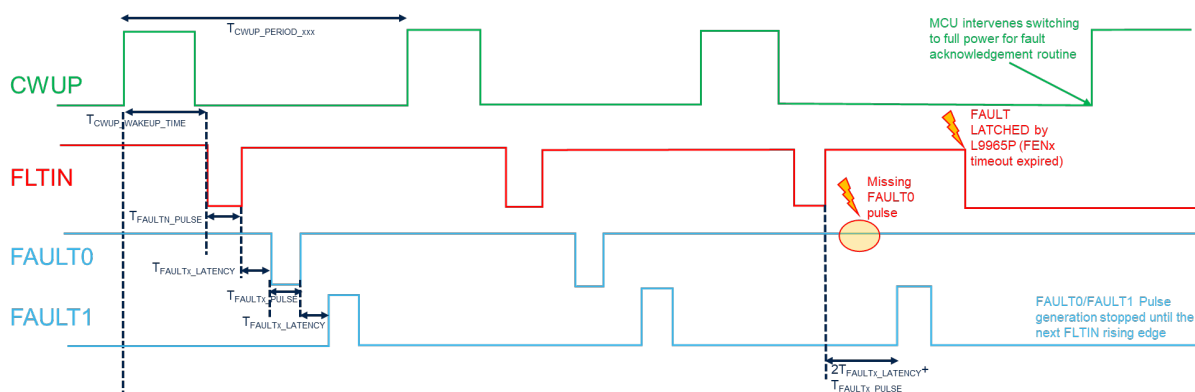
Figure 15. FAULTx lines integrity check in level mode
