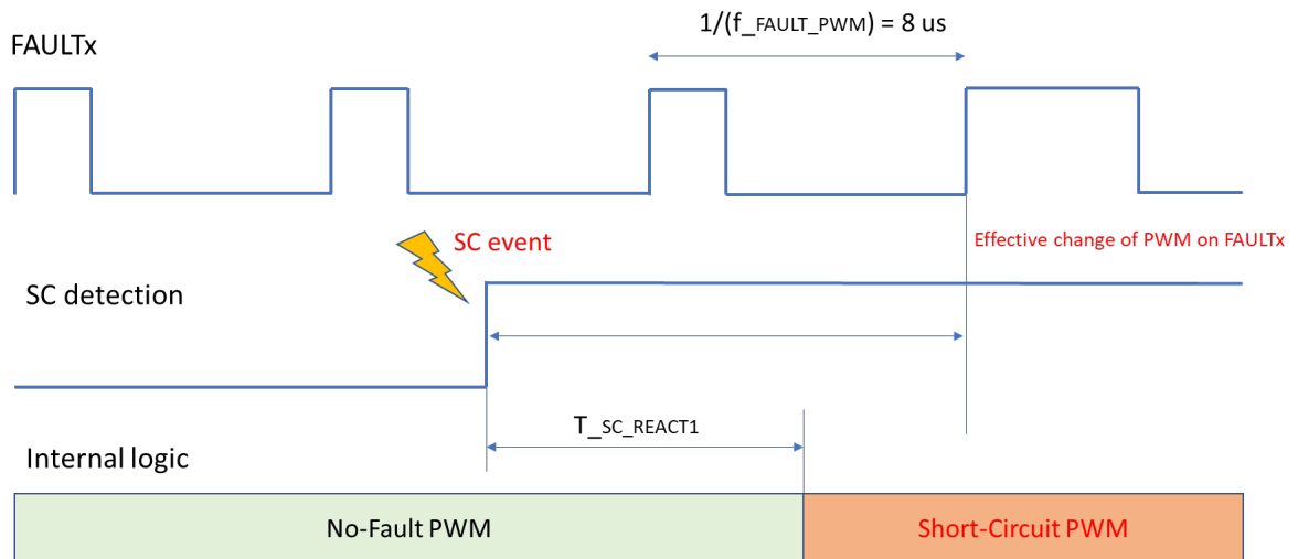
Figure 8. Short-circuit reaction time with FAULTx_MODE=1
