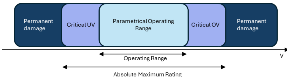
Figure 4. Pin voltage ranges
