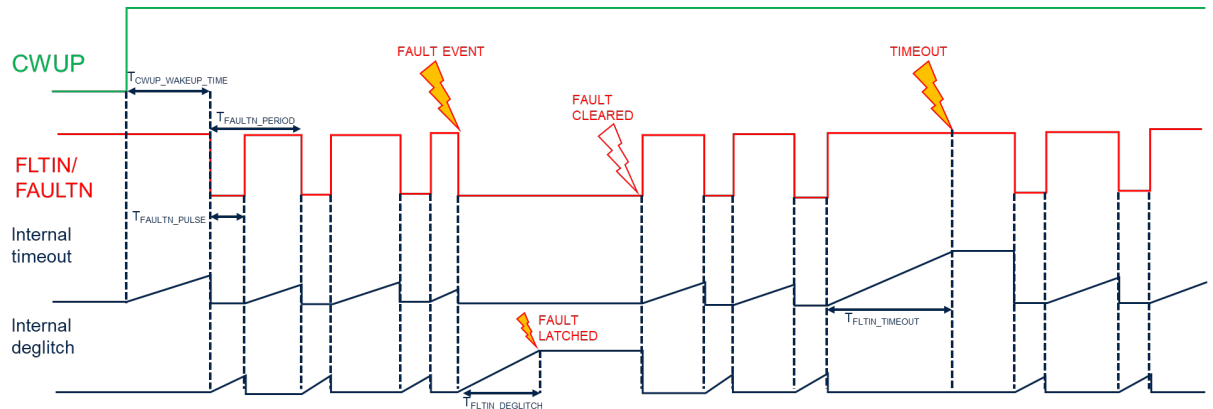
Figure 10. FLTIN integrity check in full power mode
