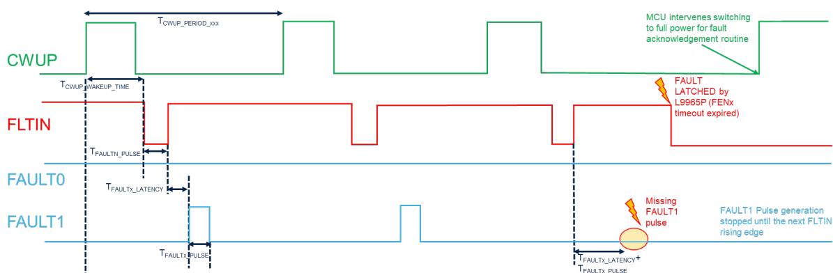
Figure 16. FAULTx lines integrity check in level mode (example with FAULT0 cyclic BIST disabled)
