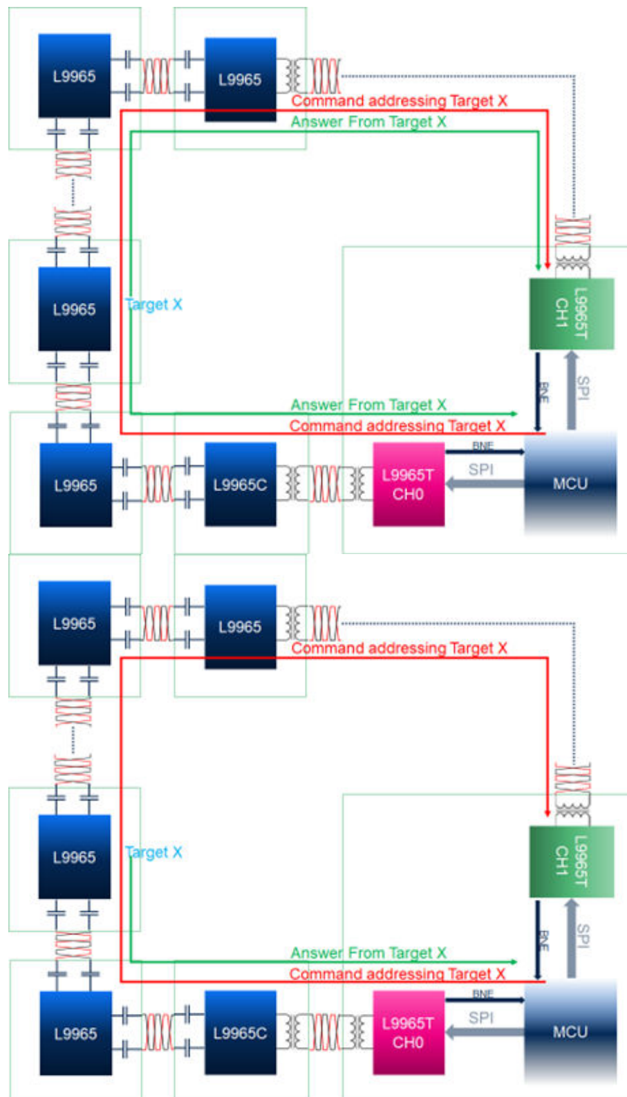
Figure 20. Bidirectional answer (top) and Monodirectional answer (bottom)
