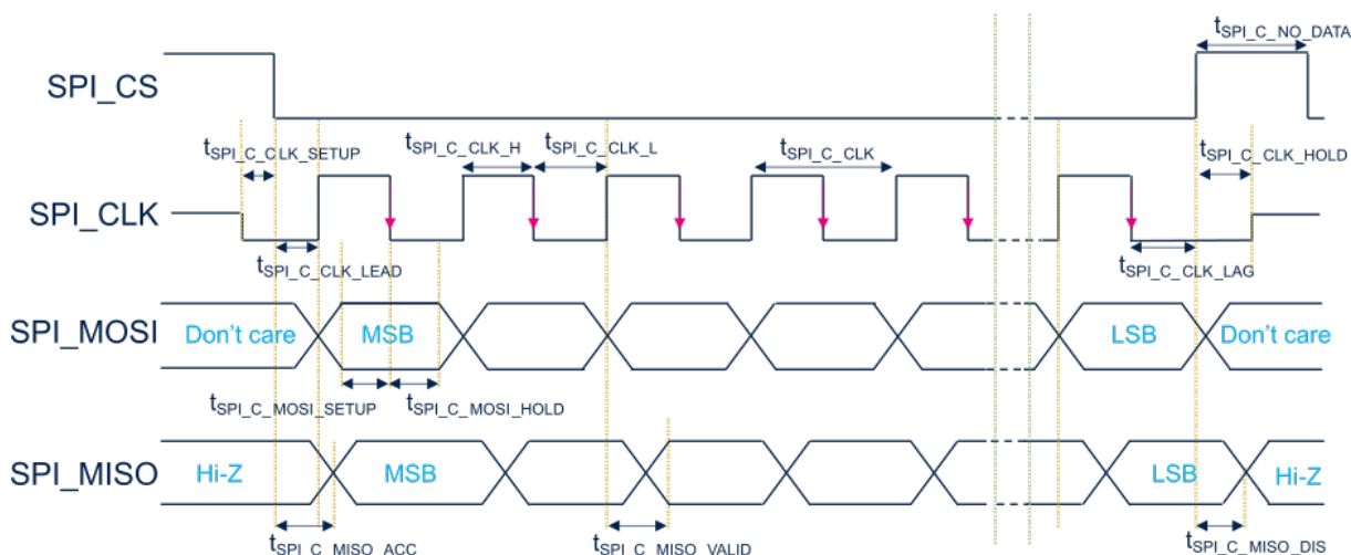
Figure 26. SPI Controller timing diagram (example with CPOL = 0 & CPHA = 1)
