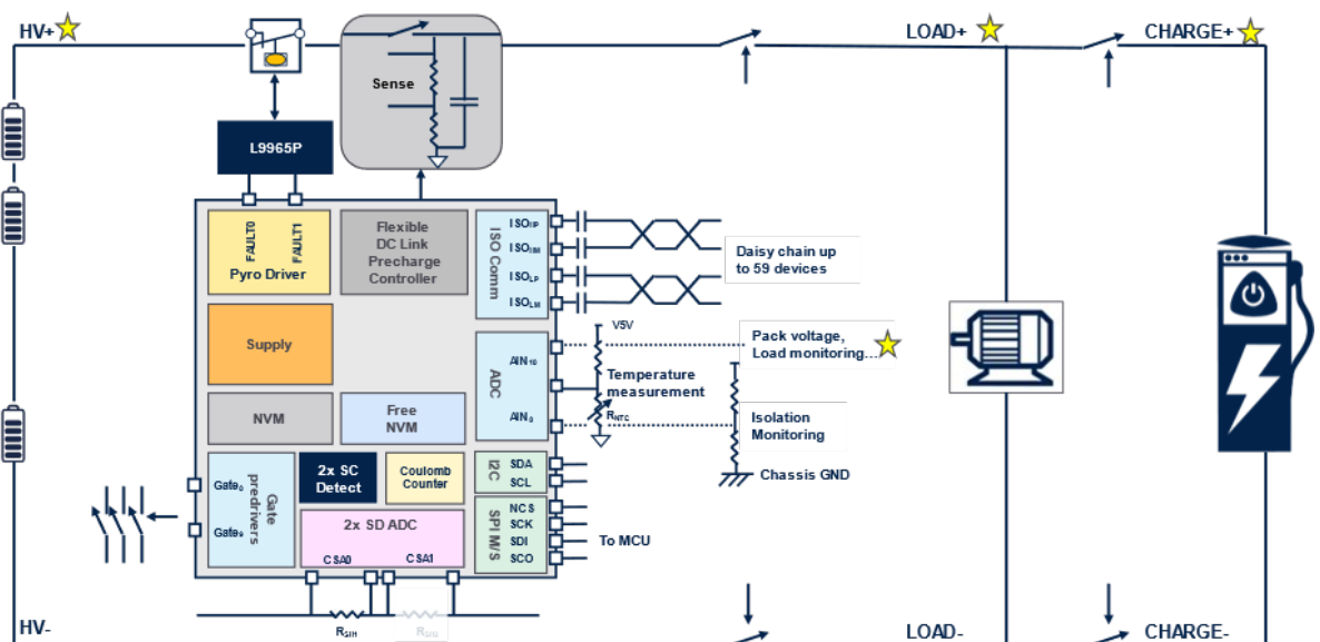
Figure 1. L9965C battery pack controller
