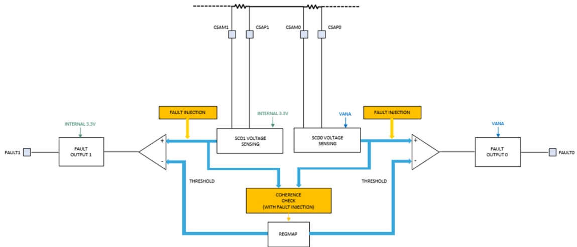
Figure 7. Fault injection principle
