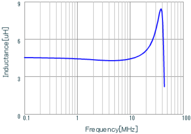
LQH44PZ4R7MGR L
