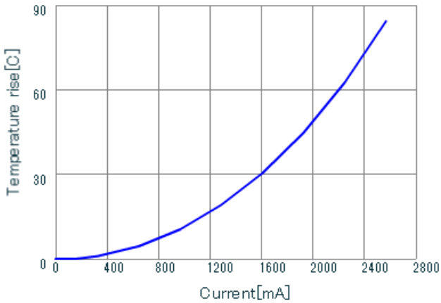
LQH44PZ4R7MGR DT_Current
