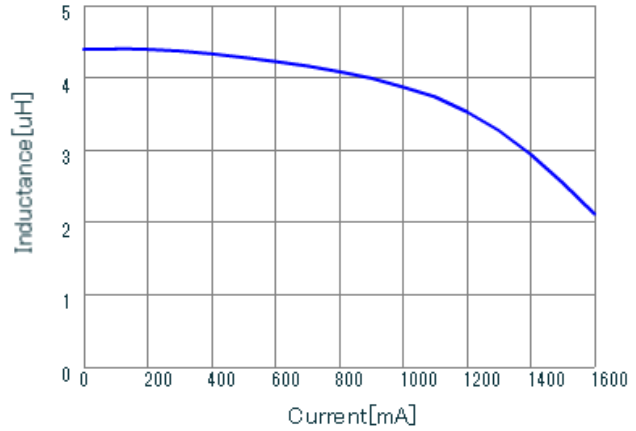
LQH44PZ4R7MGR DC-Bias, 20
