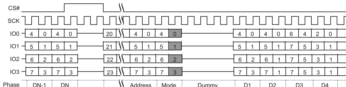
Figure 49. Fast Read Quad I/O Command Sequence (Previous command set M5-4 = 10)
