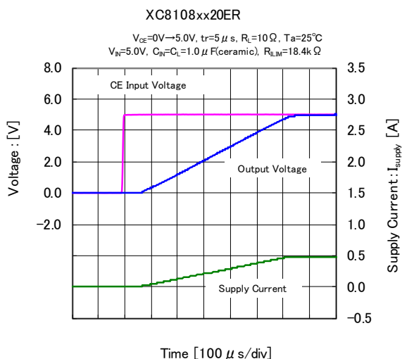
(16) turn-on Delay vs. Rise Time ( C_L=1.0\mu F )
