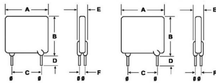
Fig.1 Lead Size : 20AWG Φ0.81 mm Diameter
