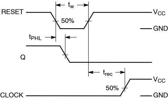
Figure 4. Switching Waveform
