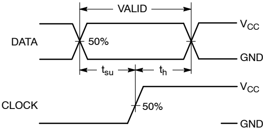
Figure 5. Switching Waveform
