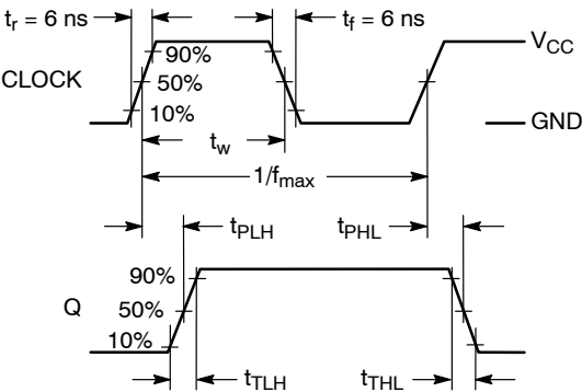
Figure 3. Switching Waveform
