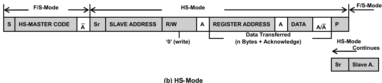
Figure 34. Data Transfer Format in F/S Mode and H/S Mode
