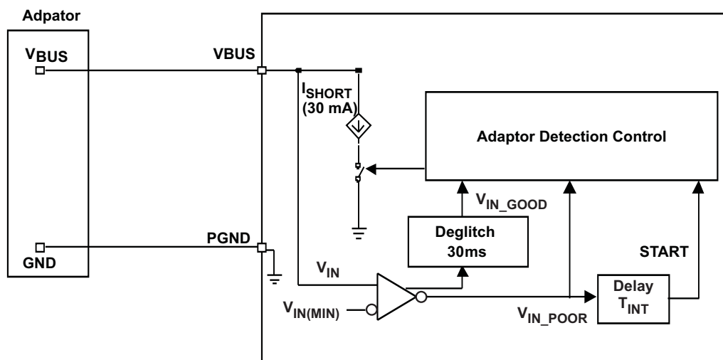
Figure 28. Bad Adaptor Detection Circuit
