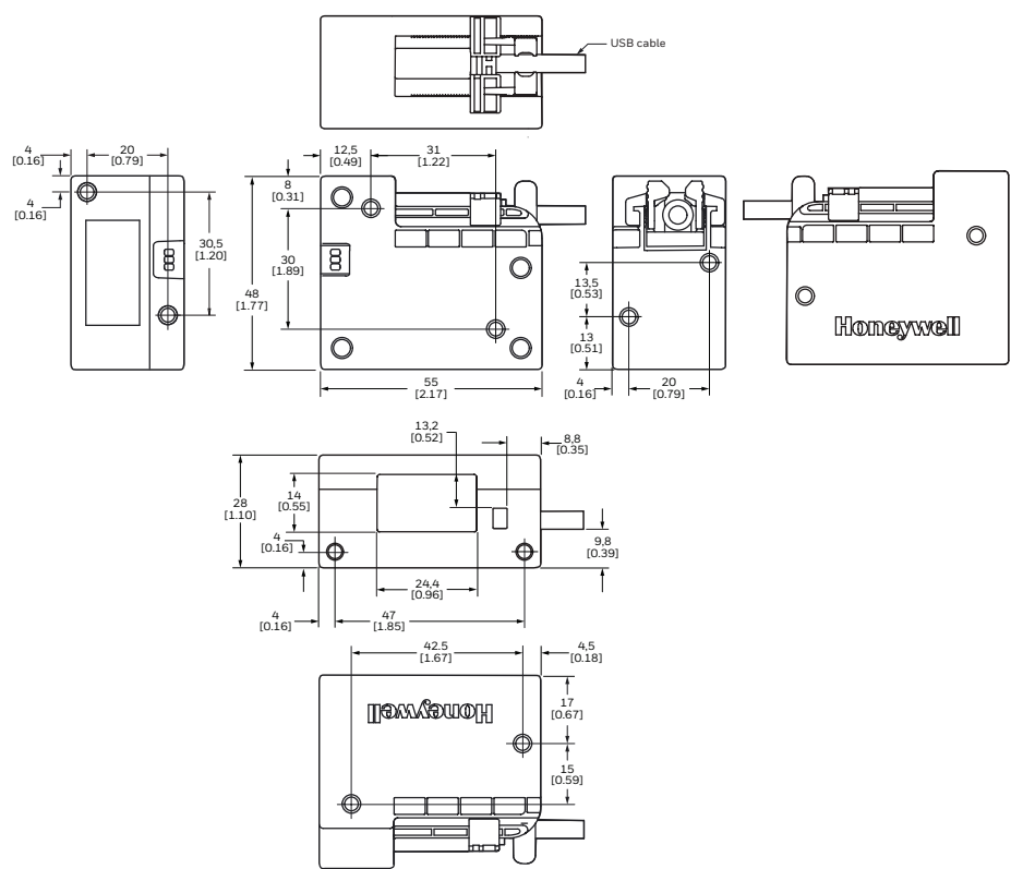
FIGURE 3. MOUNTING AND DIMENSIONAL DRAWING (FOR REFERENCE ONLY: MM/[IN])
