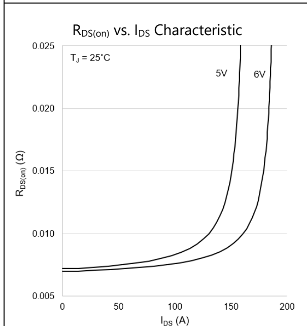
Figure 3: R_{DS(on)} vs. I_{DS} at T_J = 25^\circ\text{C}
