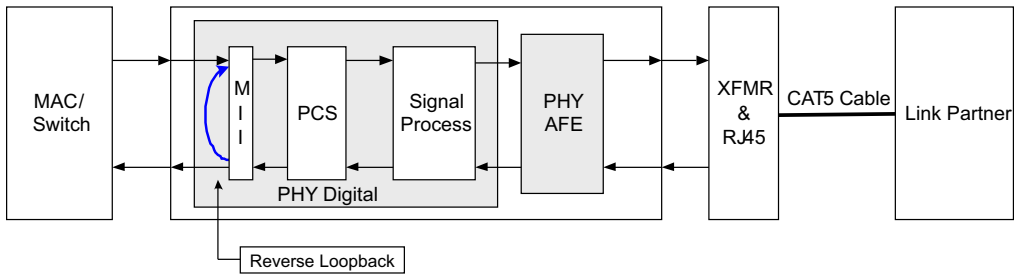
Figure 3-6. Block Diagram, Far-End Loopback Mode
