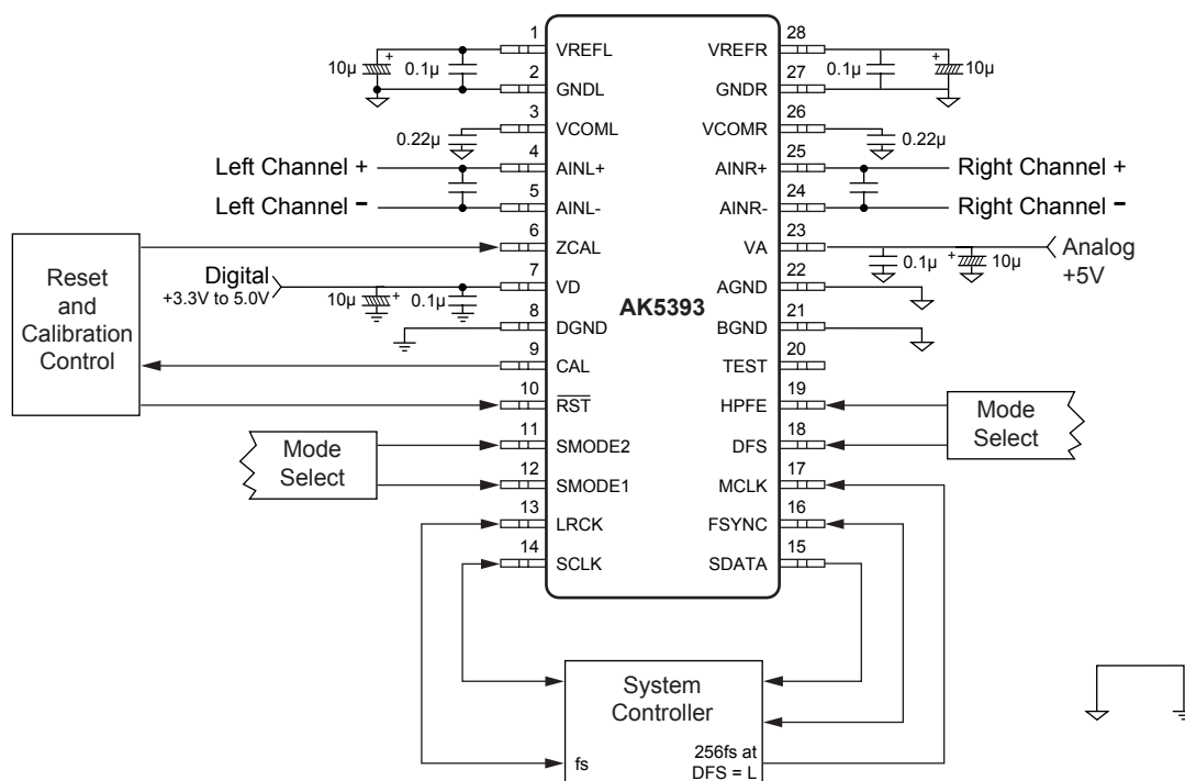
Figure 10. Typical Connection Diagram for Crystal Mode
