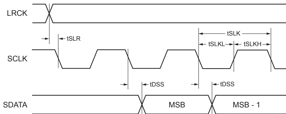
Figure 3. Serial Data Timing (I²S Slave Mode, FSYNC = Don't Care)
