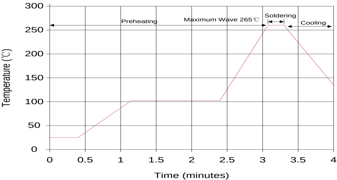
Lead-free Wave Soldering Recommendation
