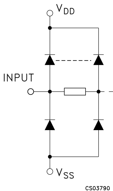
Figure 1. Inputand equivalent circuit diagram
