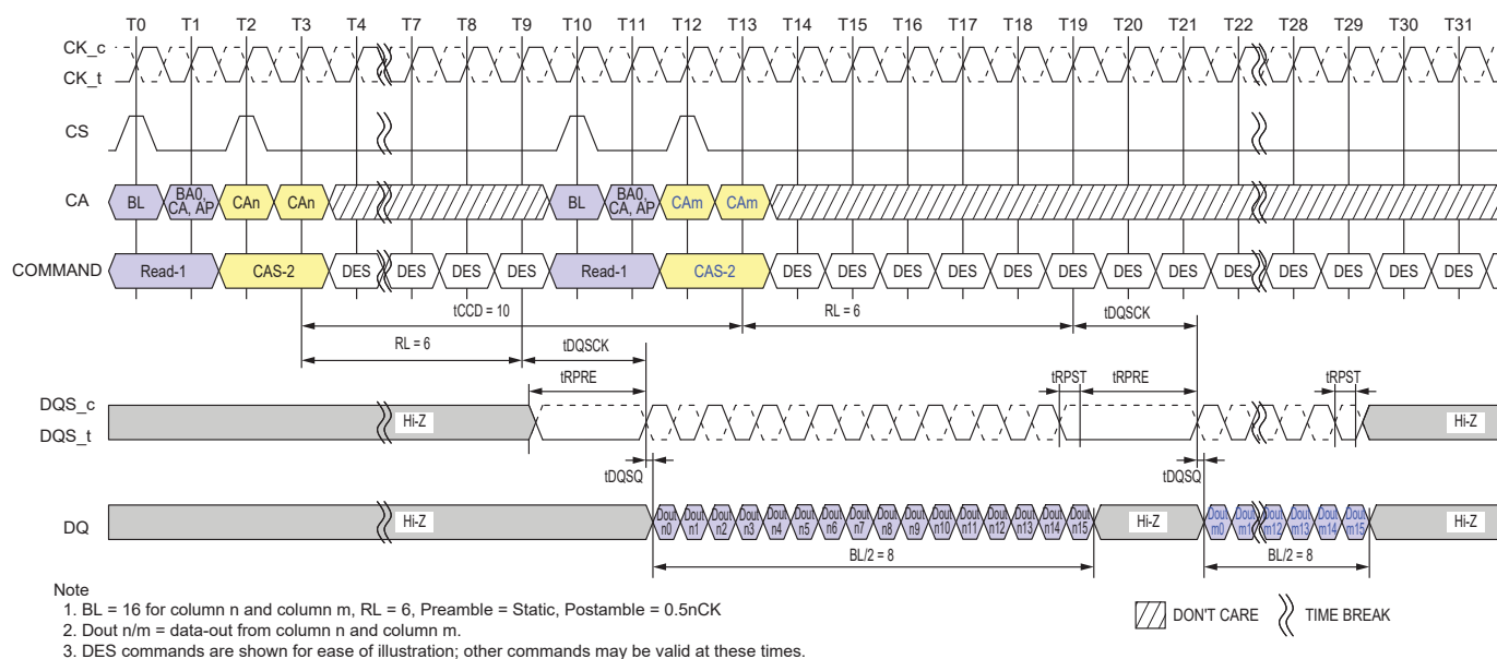
Figure 4.27 — Consecutive Reads Operation: tCCD = Min +2, Preamble = Static, 0.5nCK Postamble
