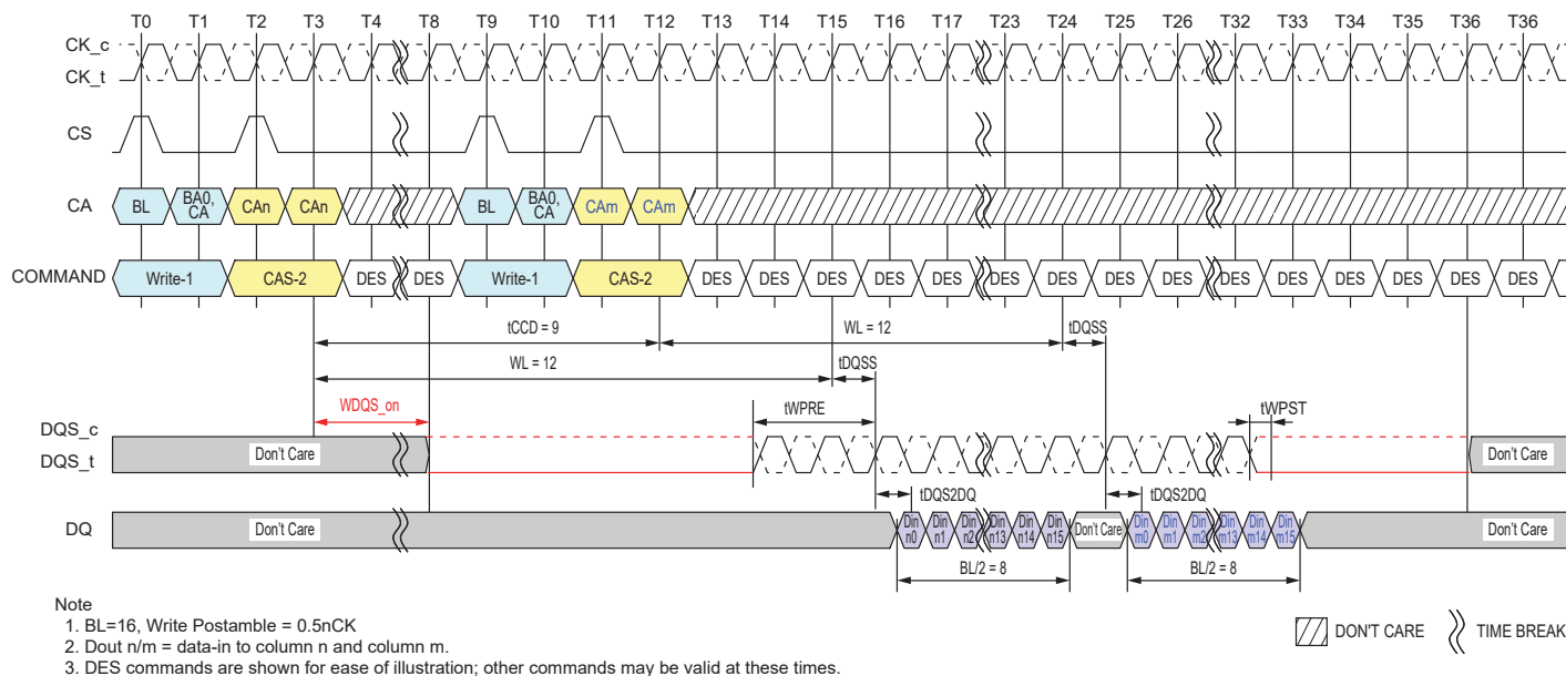
Figure 4.35 — Consecutive Writes Operation: t_{CCD} = \text{Min} + 1, 0.5\text{nCK} Postamble
