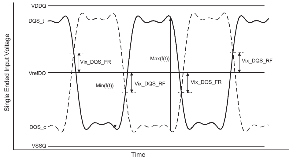
Figure 7.12 — DQS input Crosspoint voltage (Vix) Table 7.16 — DQS input voltage crosspoint(Vix) ratio
