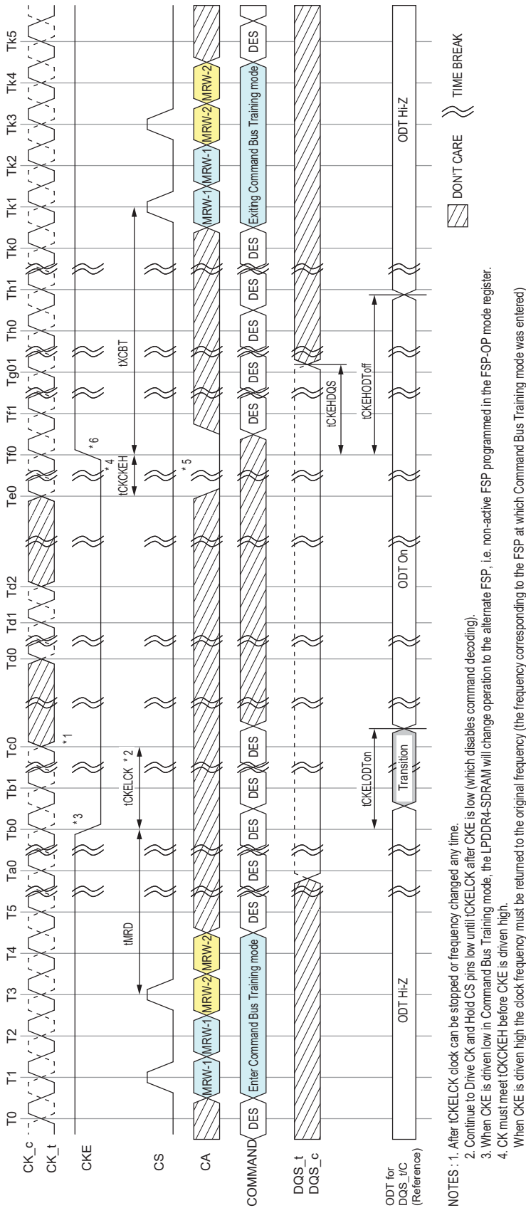
4.25.2.2.4 Timing Diagram for mode 2 (Cont'd)
