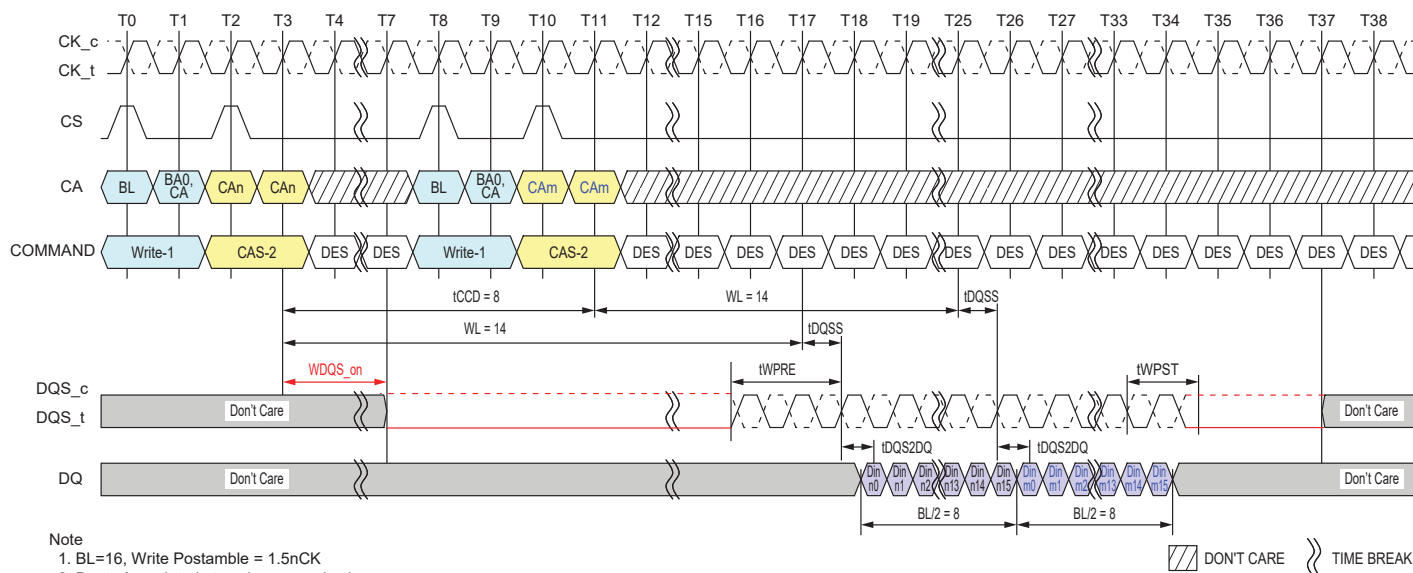
Figure 4.34 — Seamless Writes Operation: t_{CCD} = \text{Min}, 1.5\text{nCK} Postamble
