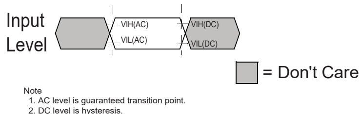
Figure 7.1a — Input Timing Definition for CKE
