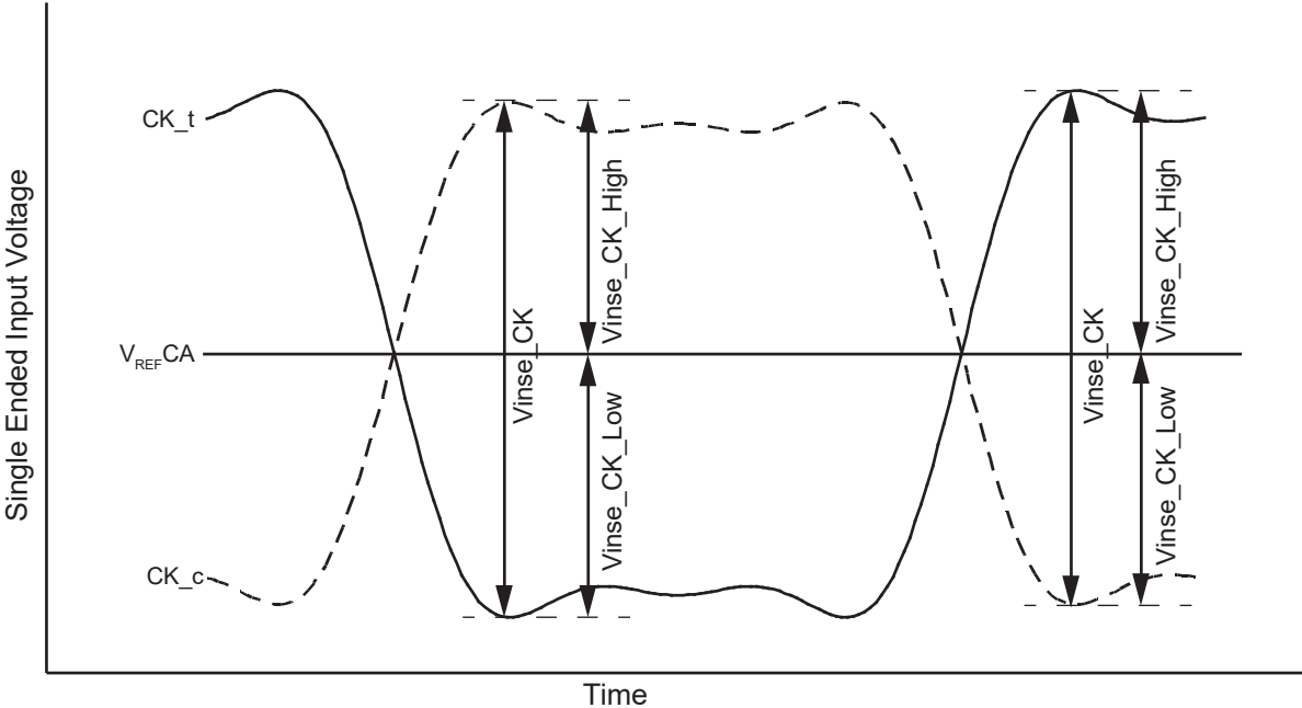
Figure 7.5 — Clock Single-Ended Input Voltage
