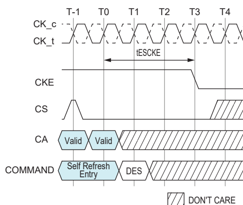
Figure 4.59 — tESCCKE Timing
