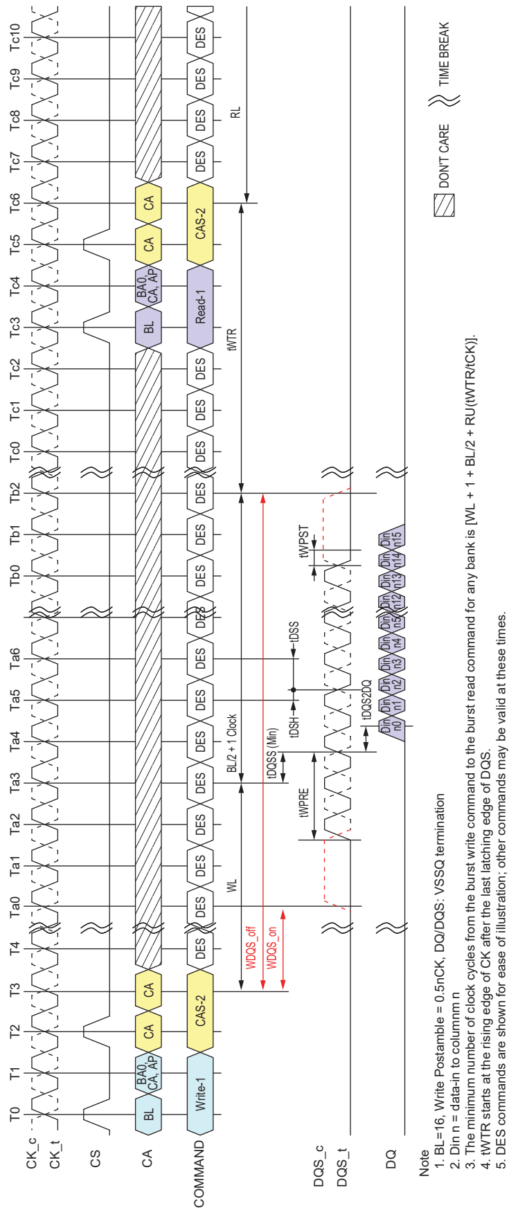
Figure 4.15 — Burst Write Followed by Burst Read
