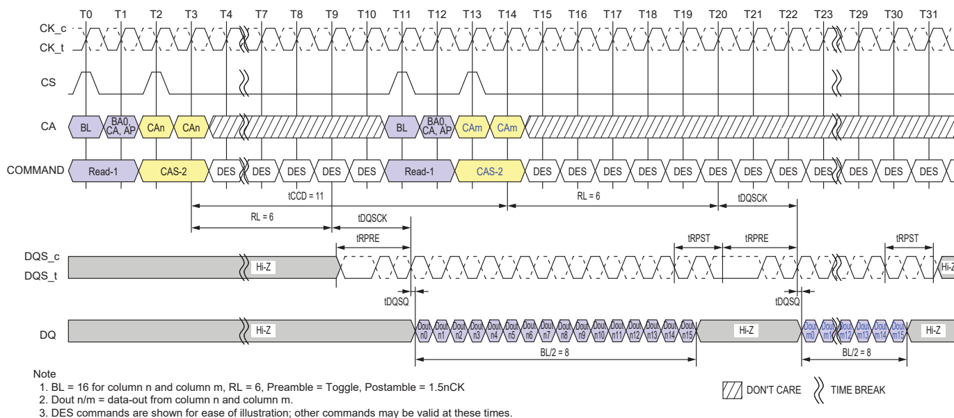
Figure 4.28 — Consecutive Reads Operation: tCCD = Min +3, Preamble = Toggle, 1.5nCK Postamble
