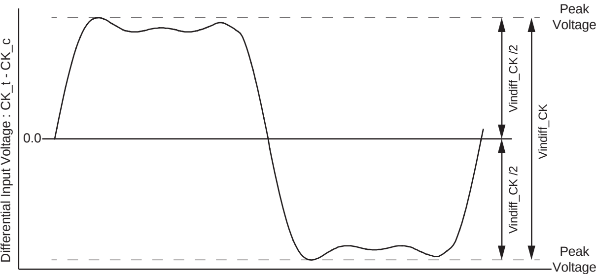
Figure 7.3 — CK Differential Input Voltage
