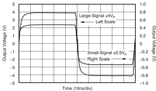
SMALL-SIGNAL AND LARGE-SIGNAL PULSE RESPONSES
