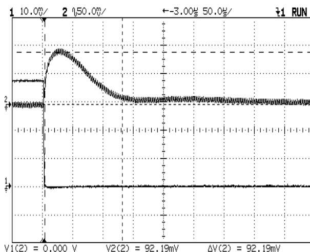
EHS15-033 Transient Response 50- 25% step, 1A/μs
