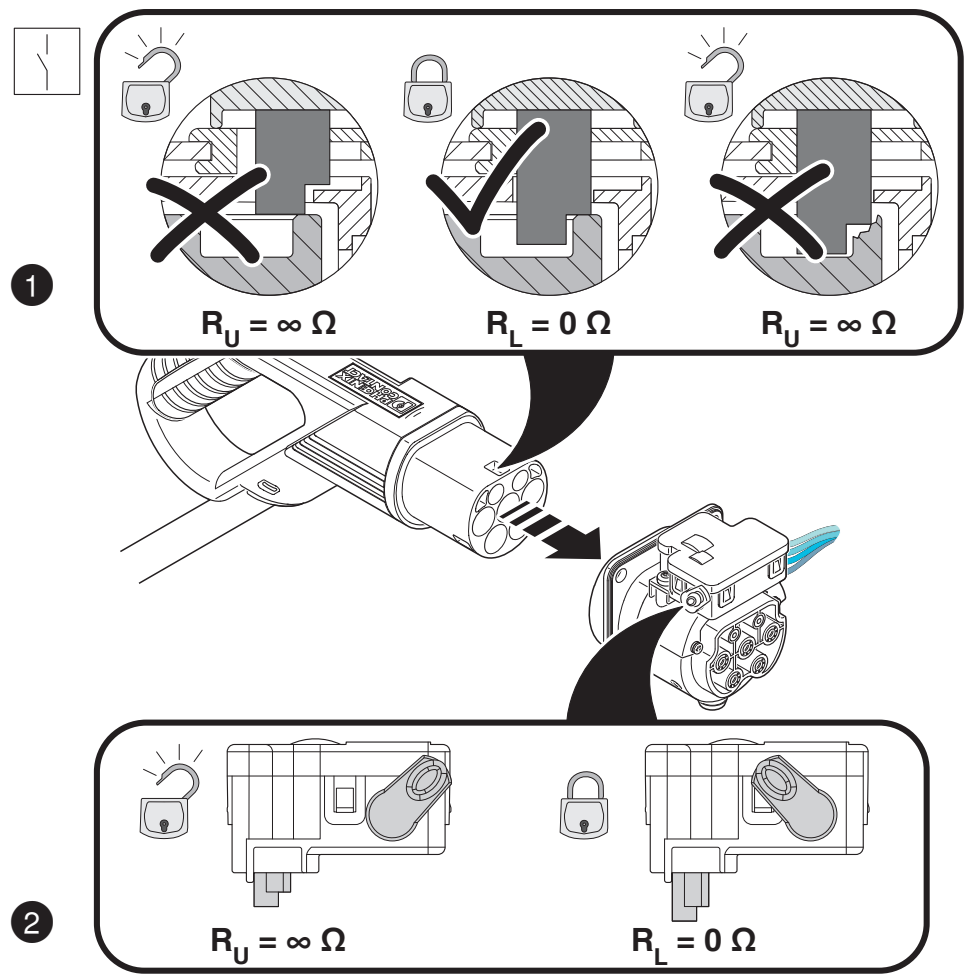
Schematic diagram
