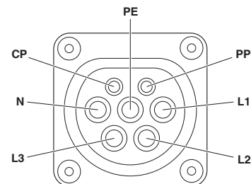
Connection diagram
