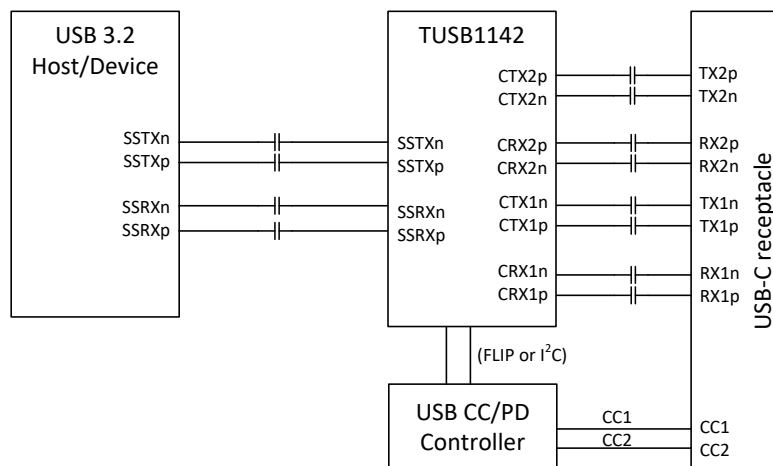
Simplified Schematic
