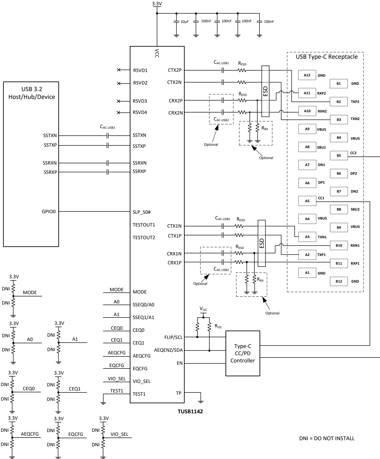
Figure 11-1. Application Circuit
