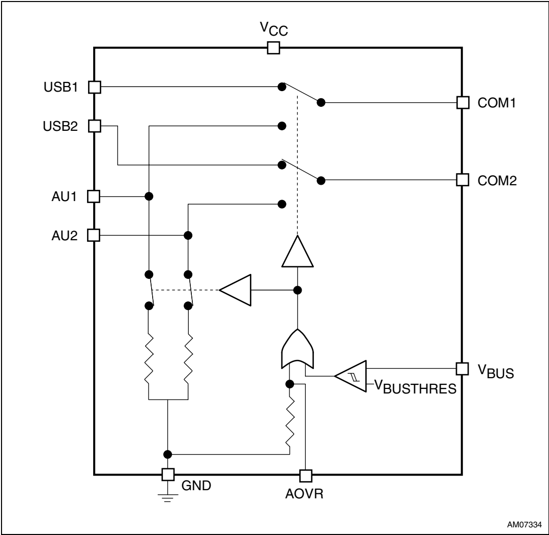
Figure 3. Functional diagram
