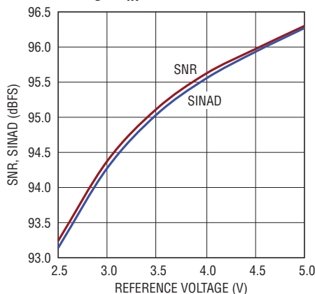
SNR, SINAD vs Reference Voltage, f_{IN} = 2\text{kHz}
