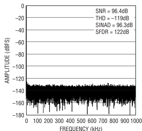
32k Point FFT f_s = 2\text{Msps} , f_{\text{IN}} = 2\text{kHz}
