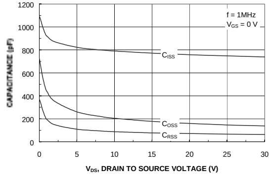
Figure 18. Capacitance Characteristics.
