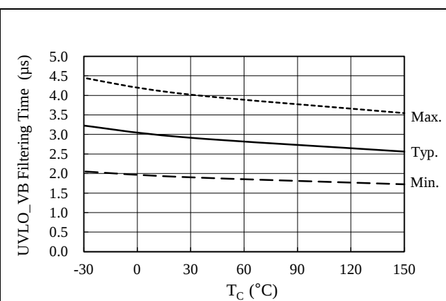
Figure 14-15. UVLO_VCC Filtering Time vs. T_C
