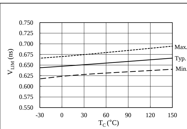
Figure 14-25. Current Limit Reference Voltage, V_{LIM} vs. T_C
