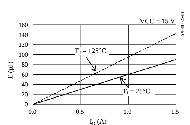
Figure 14-39. Low-side Switching Loss
