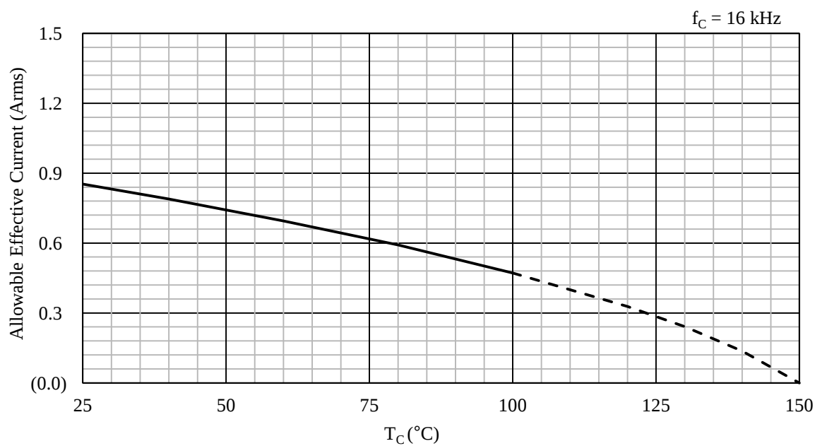
Figure 14-47. Allowable Effective Current ( f_C = 16 \text{ kHz} ): SX68003MH
