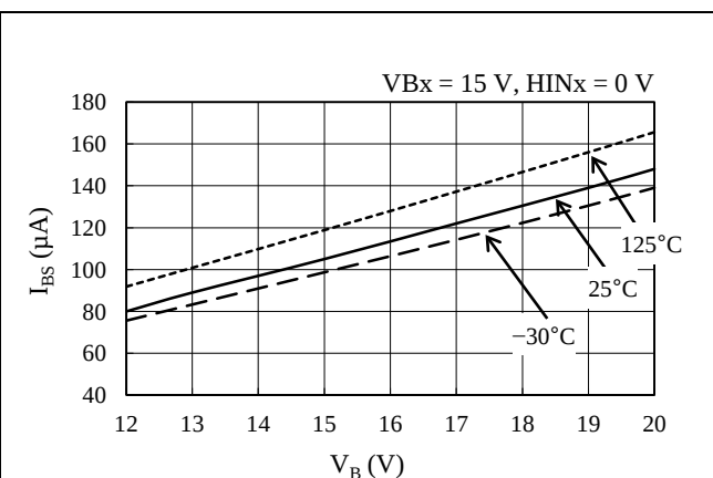
Figure 14-9. V_{Bx} Pin Voltage, V_B vs. Logic Supply Current I_{BS} curve ( H_{IN_x} = 0 V)
