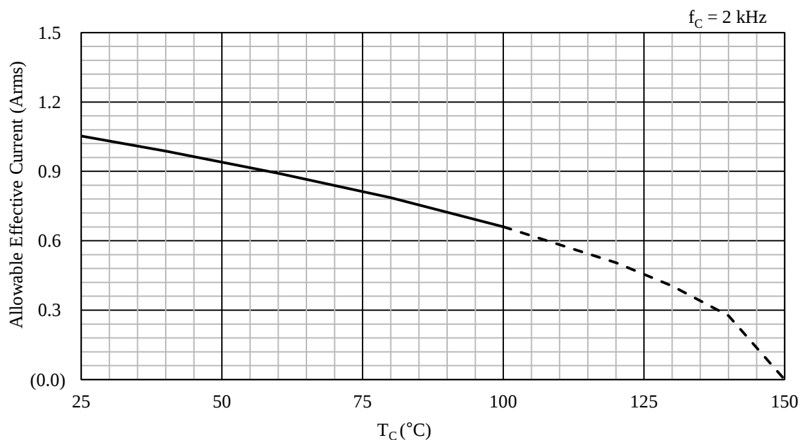
Figure 14-46. Allowable Effective Current ( f_C = 2 \text{ kHz} ): SX68003MH
