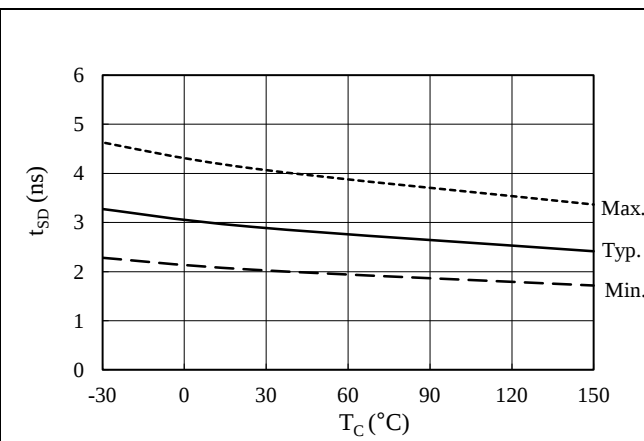
Figure 14-23. SD Pin Filtering Time vs. T_C
