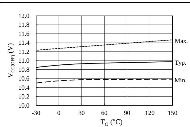
Figure 14-13. Logic Operation Stop Voltage, V_{CC(OFF)} vs. T_C
