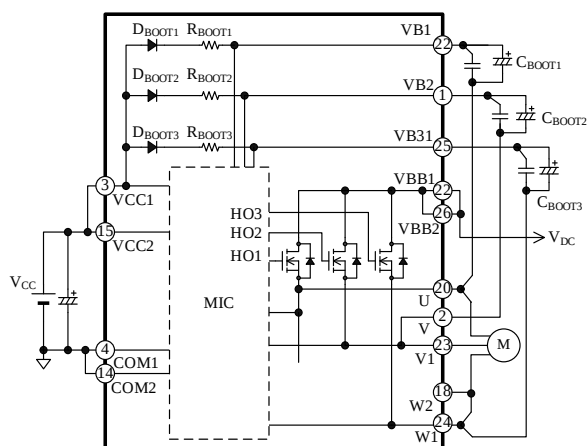
Figure 11-1. Bootstrap Circuit
