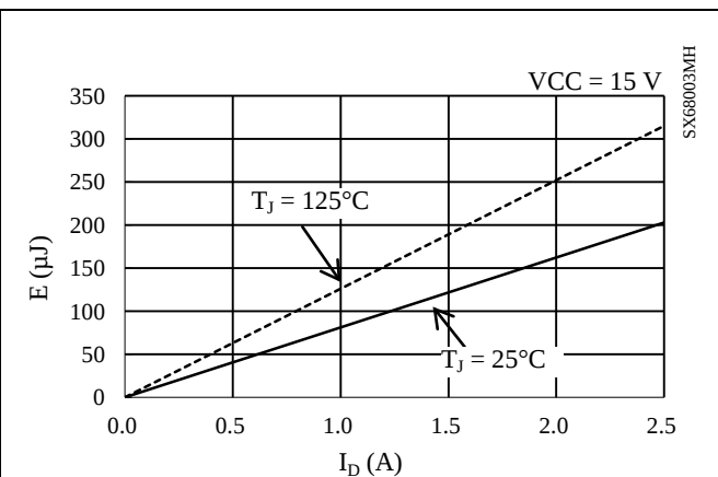
Figure 14-41. Low-side Switching Loss
