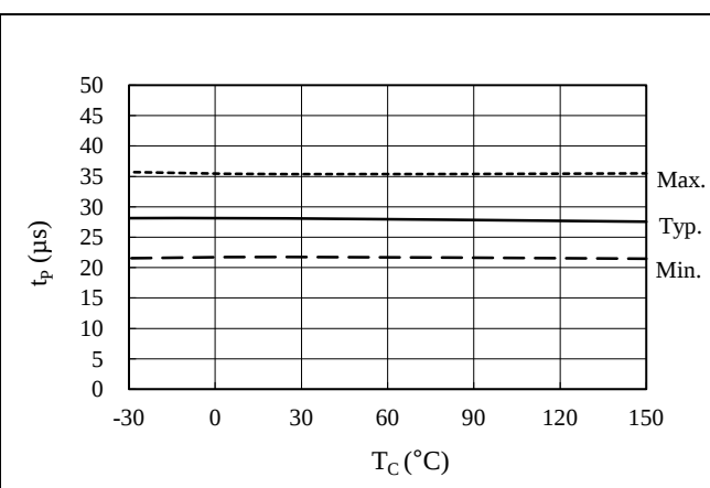
Figure 14-27. OCP Hold Time, t_p vs. T_C
