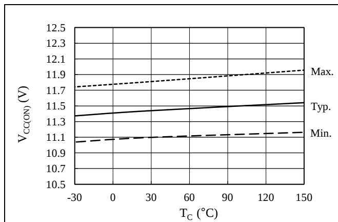
Figure 14-12. Logic Operation Start Voltage, V_{CC(ON)} vs. T_C
