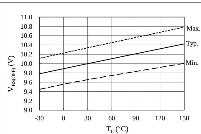
Figure 14-11. Logic Operation Stop Voltage, V_{BS(OFF)} vs. T_C
