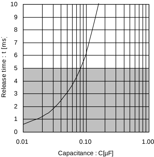
Figure 9. Release Time (Reference Data @R=100k \Omega )
