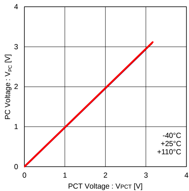
Figure 33. PCT vs PC Linearity ( R_{PCT}=R_{PC}=100k\Omega )
