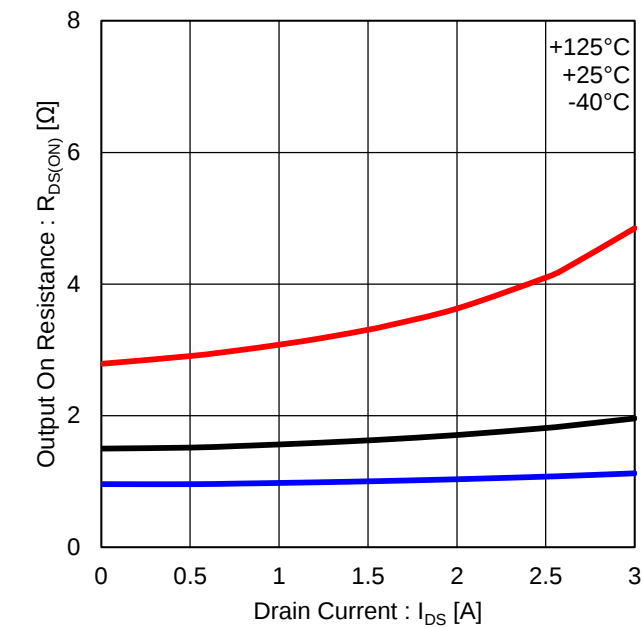
Figure 18. Output MOSFET ON Resistance
