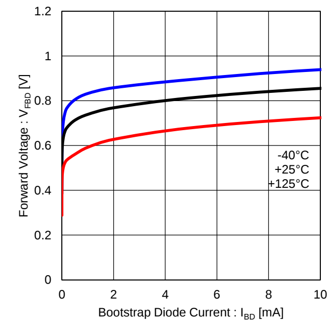
Figure 20. Bootstrap Diode Forward Voltage
