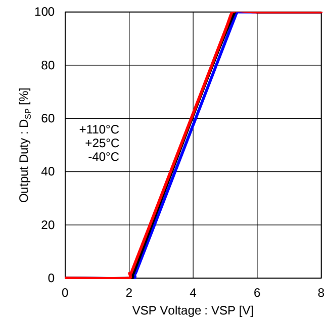
Figure 30. Output Duty vs VSP Voltage
