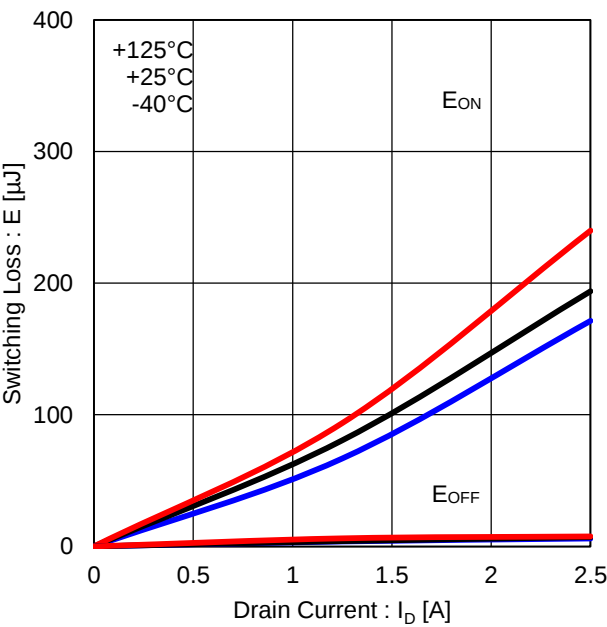
Figure 24. Low Side Switching Loss (VDC=300V)
