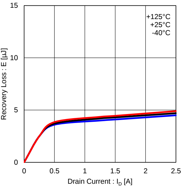
Figure 23. High Side Recovery Loss (VDC=300V)
