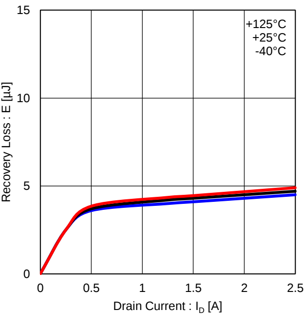
Figure 25. Low Side Recovery Loss (VDC=300V)
