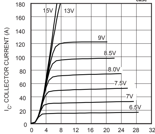
FIGURE 4, Output Characteristics ( T_J = 25^{\circ}C )
