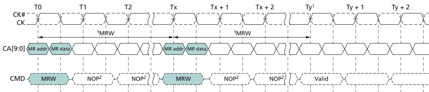
Figure 52: MODE REGISTER WRITE Timing – RL = 3, t_{MRW} = 5
