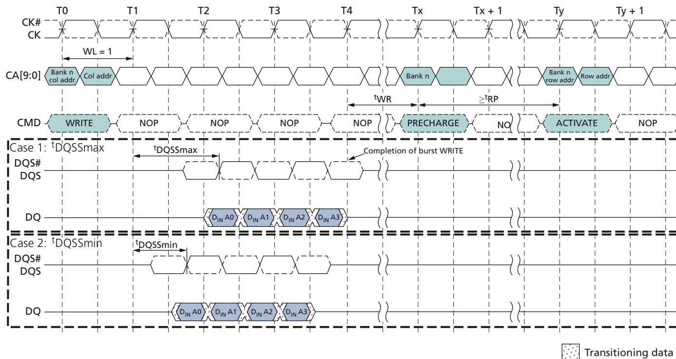
Figure 36: WRITE Burst Followed by PRECHARGE – WL = 1, BL = 4
