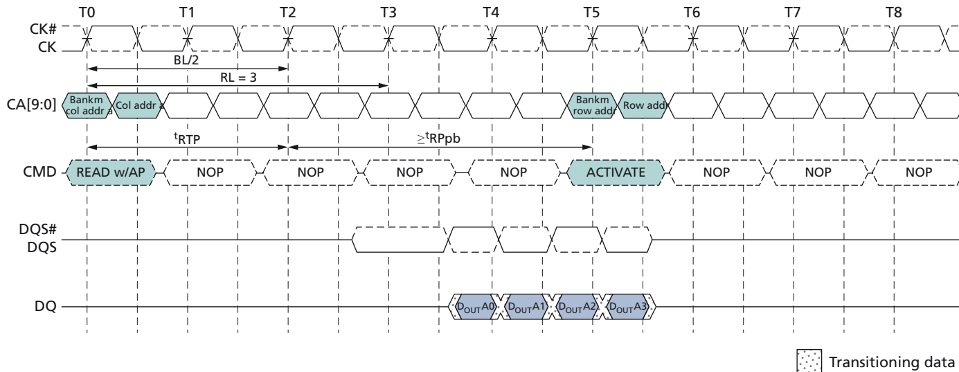
Figure 37: READ Burst with Auto Precharge – RL = 3, BL = 4, RU(t_{RTP(MIN)}/t_{CK}) = 2
