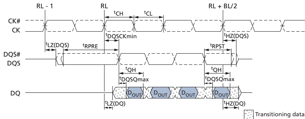
Figure 16: READ Output Timing – t_{DQSCK} (MIN)
