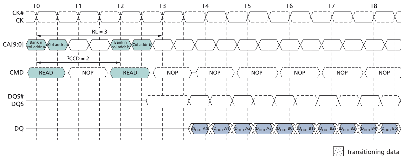
Figure 24: READ Burst Interrupt Example – RL = 3 , BL = 8 , t_{CCD} = 2
