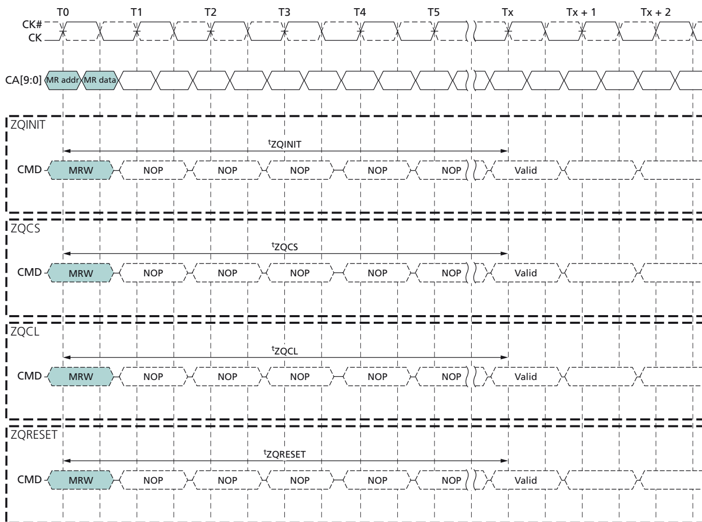
Figure 53: ZQ Timings
