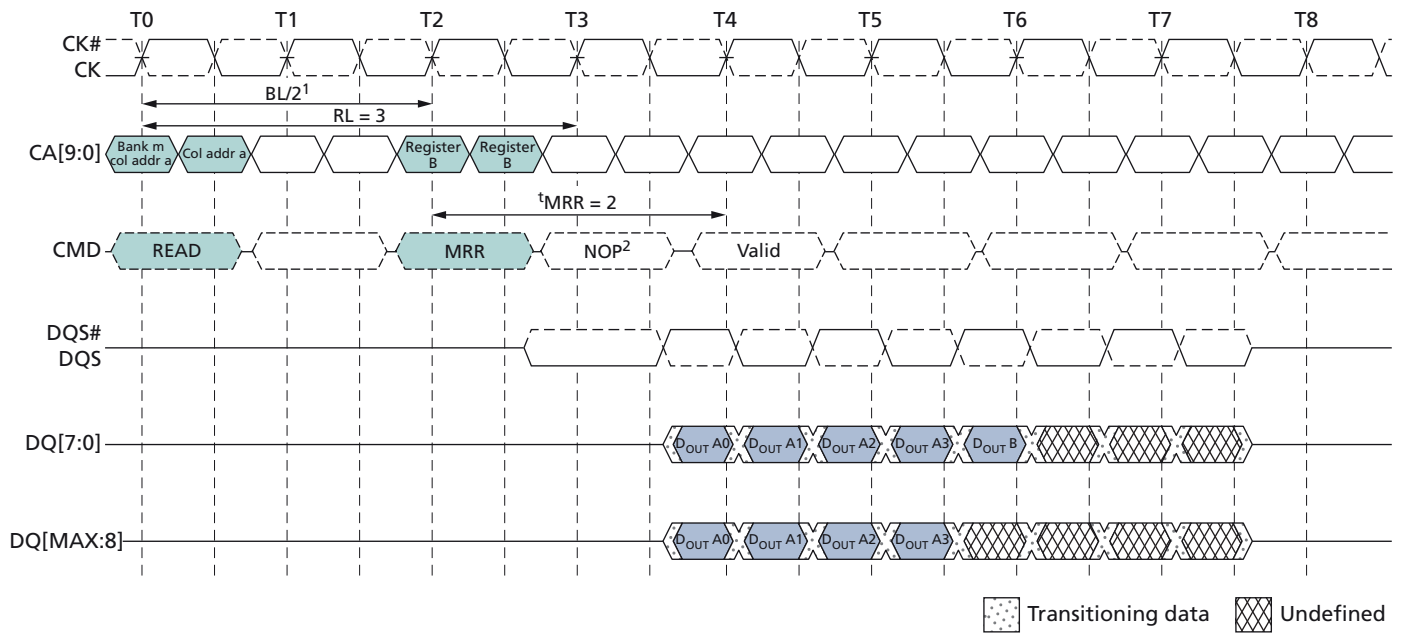
Figure 48: READ to MRR Timing – RL = 3, t_{MRR} = 2
