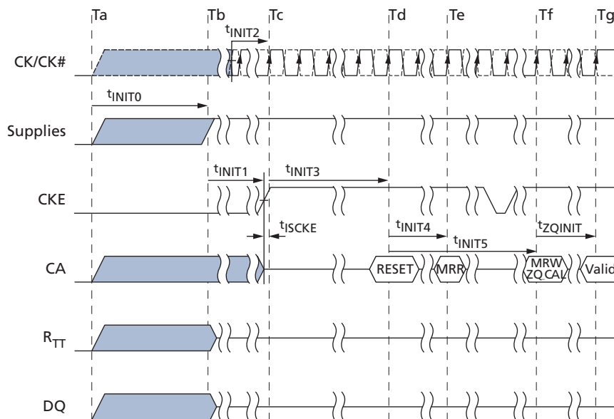
Figure 12: Voltage Ramp and Initialization Sequence
