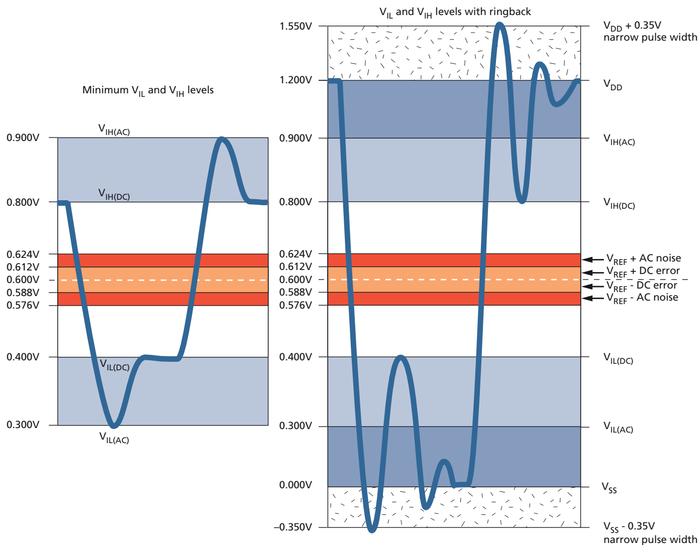
Figure 70: LPDDR2-200 to LPDDR2-400 Input Signal
