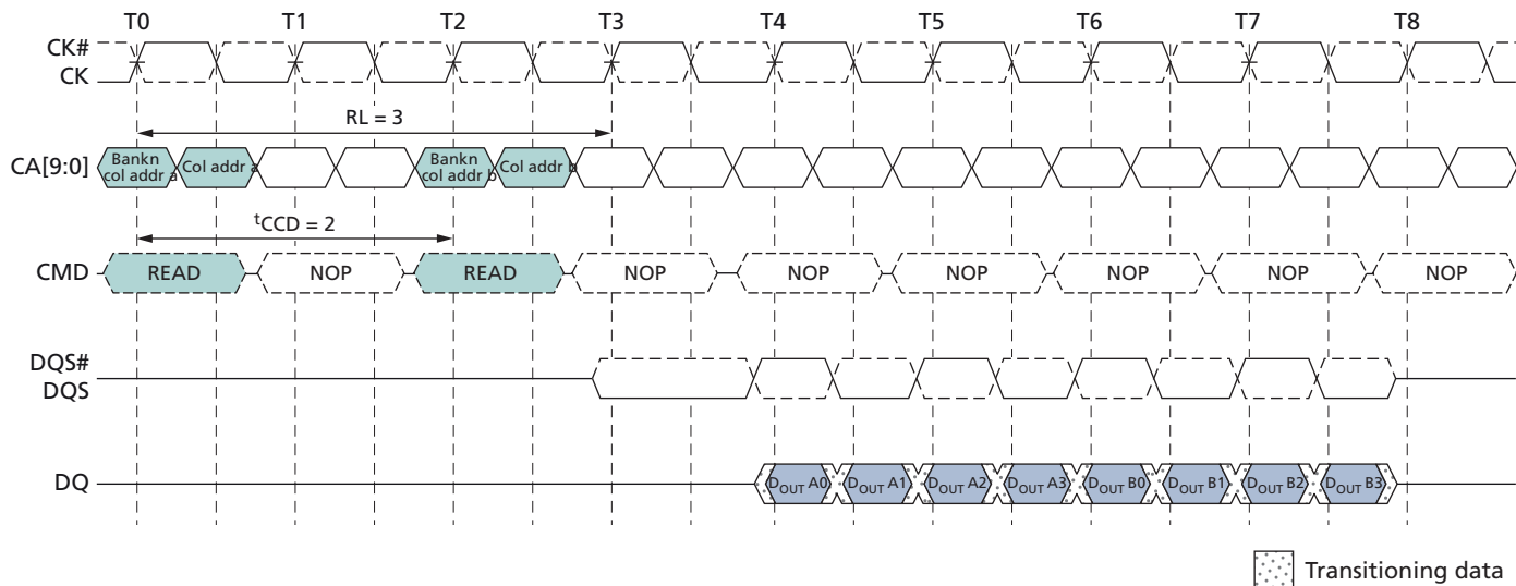
Figure 23: Seamless Burst READ – RL = 3, BL = 4, t_{CCD} = 2
