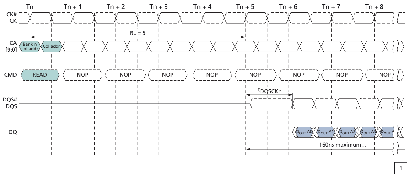
Figure 21: t_{DQCKDS} Timing
