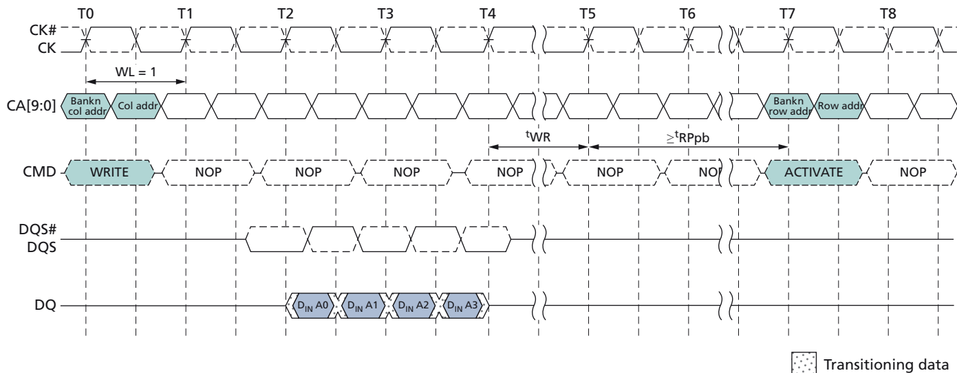
Figure 38: WRITE Burst with Auto Precharge – WL = 1, BL = 4
