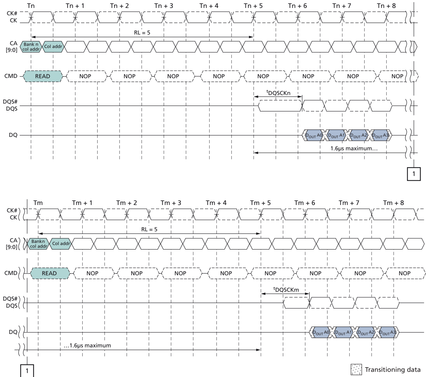
Figure 20: t_{DQSCDM} Timing
