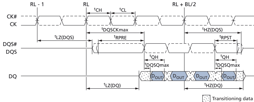
Figure 15: READ Output Timing – t_{DQSCK} (MAX)
