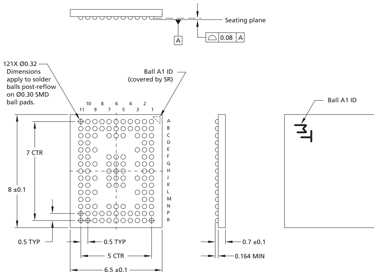
Figure 5: 121-Ball FBGA – 6.5mm x 8mm (Package Codes AB, FE)
