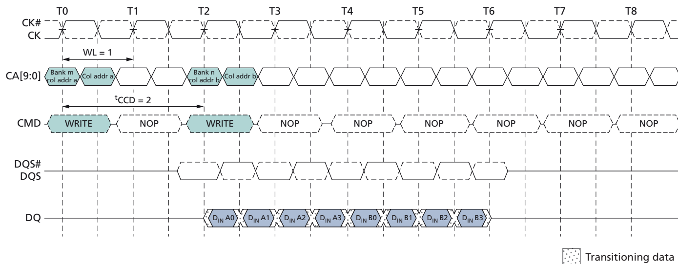
Figure 28: Seamless Burst WRITE – WL = 1, BL = 4, t_{CCD} = 2
