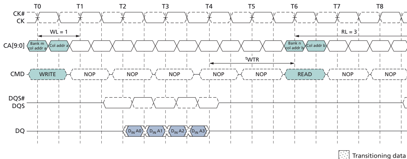
Figure 27: Burst WRITE Followed by Burst READ – RL = 3, WL = 1, BL = 4
