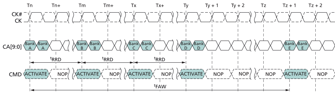
Figure 14: t_{FAW} Timing (8-Bank Devices)
