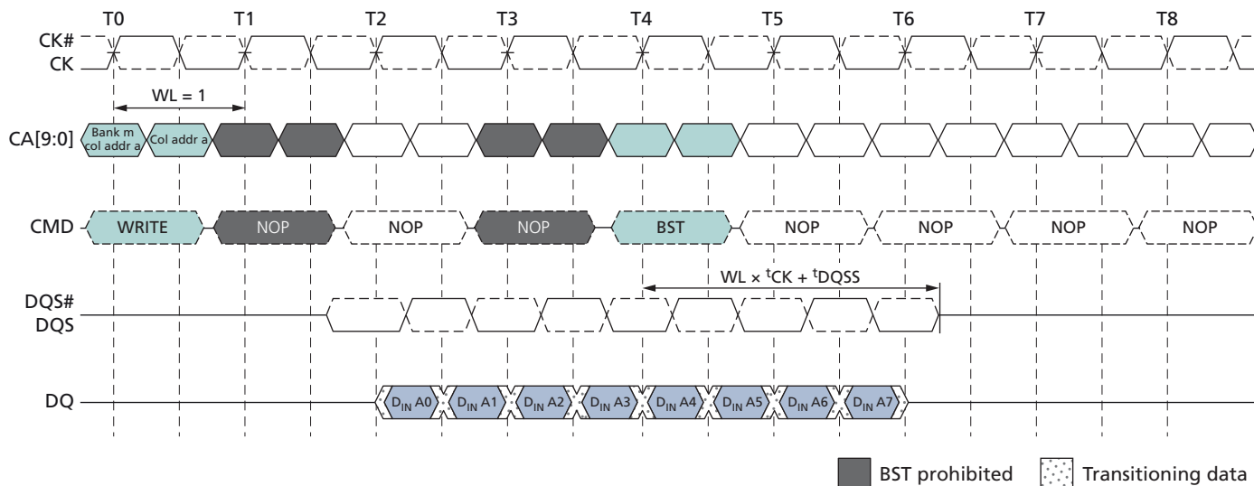
Figure 30: Burst WRITE Truncated by BST – WL = 1, BL = 16
