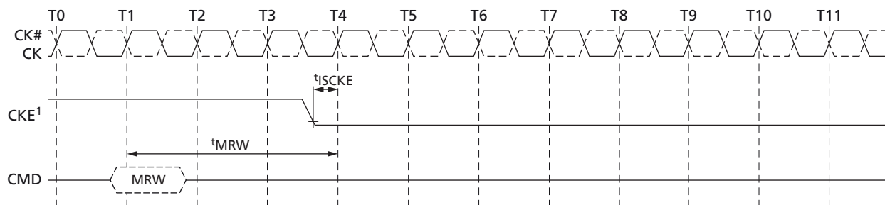
Figure 65: MRW Command to Power-Down Entry
