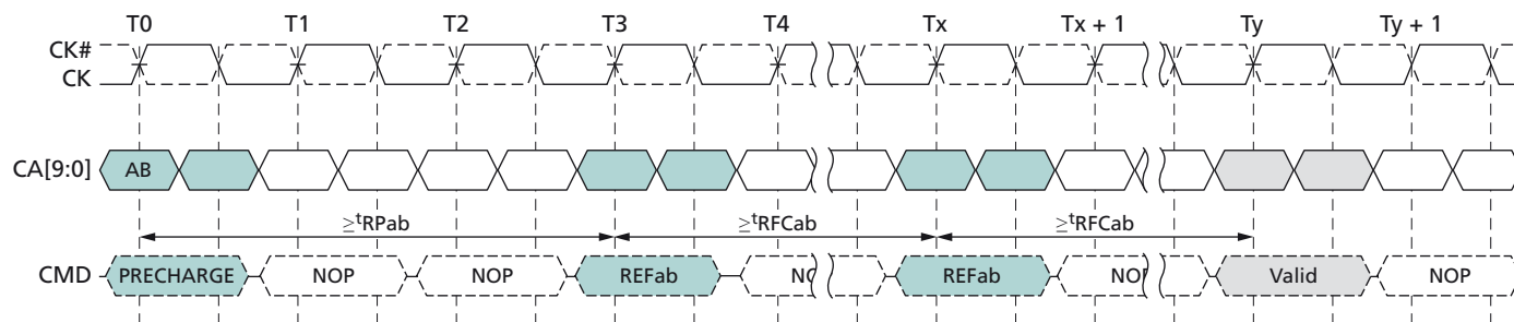
Figure 44: All-Bank REFRESH Operation
