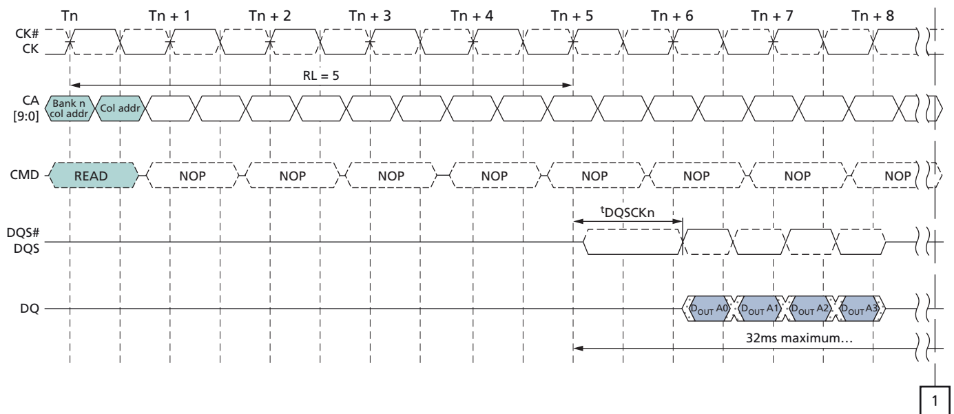
Figure 19: t_{DQSKDL} Timing
