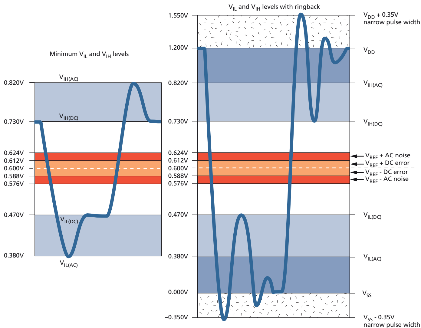
Figure 69: LPDDR2-466 to LPDDR2-1066 Input Signal
