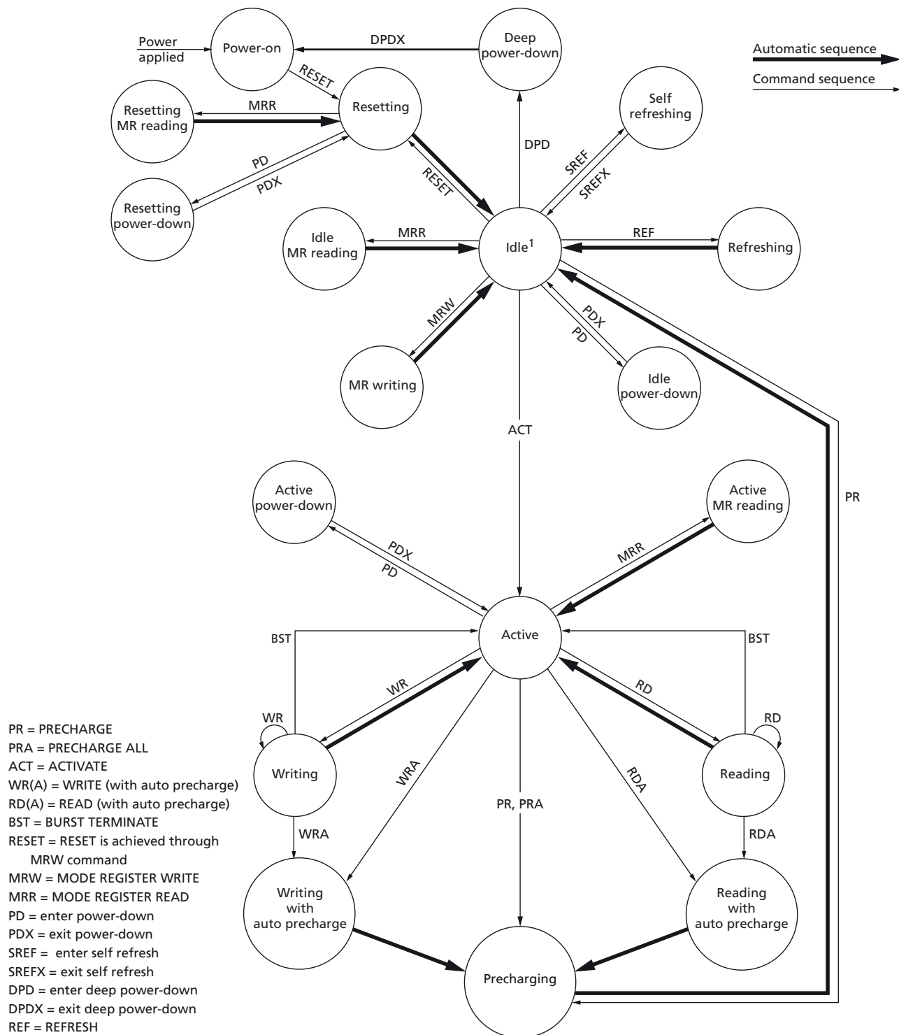
Figure 67: Simplified Bus Interface State Diagram
