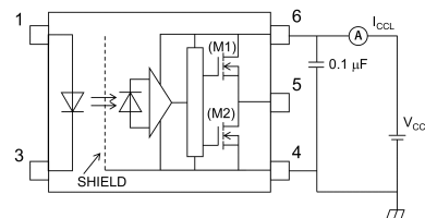
Fig. 12.1.6 I_{CCL} Test Circuit
