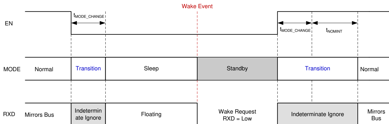
Figure 8-14. Mode Transitions
