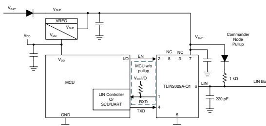
Simplified Schematics, Commander Mode
