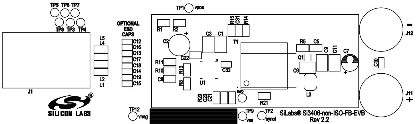
PRIMARY SILKSCREEN
