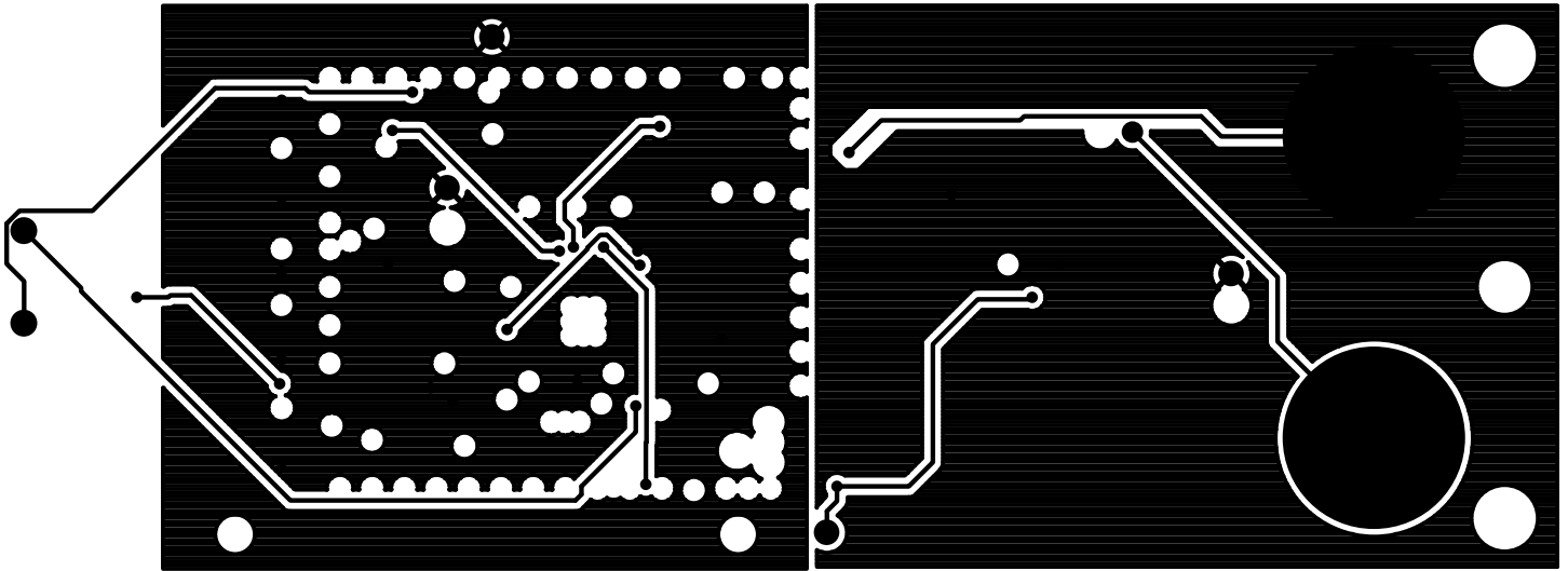
INTERNAL 1
