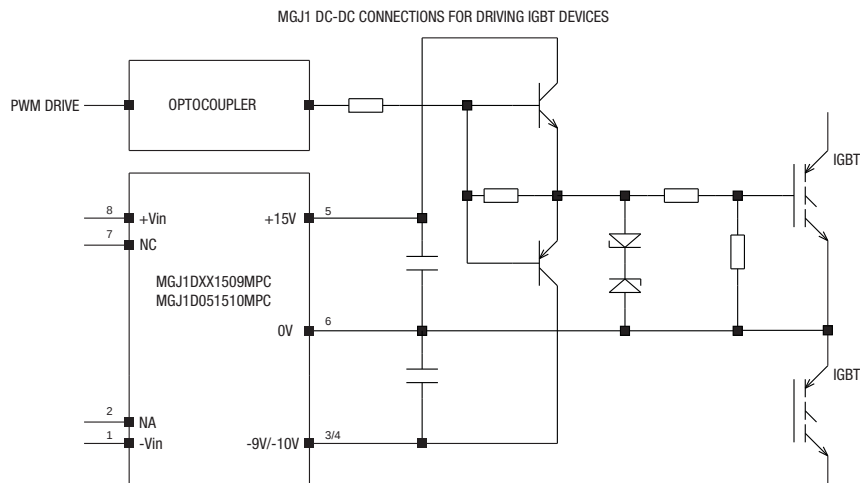
MGJ1 DC-DC CONNECTIONS FOR DRIVING SiC DEVICES
