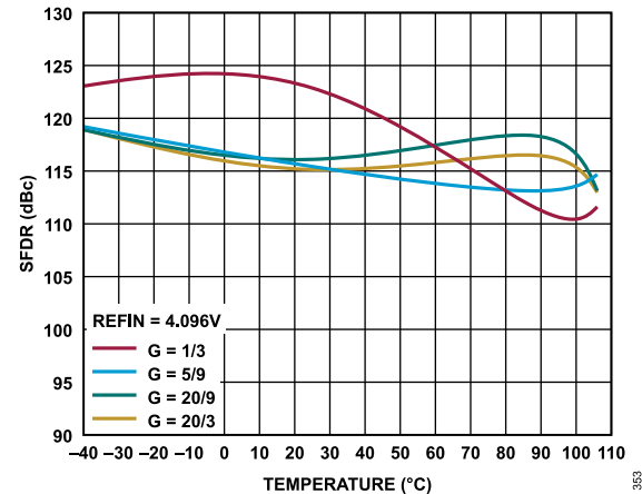
Figure 53. SFDR vs. Temperature, f_{IN} = 1 kHz, REFIN = 4.096 V
