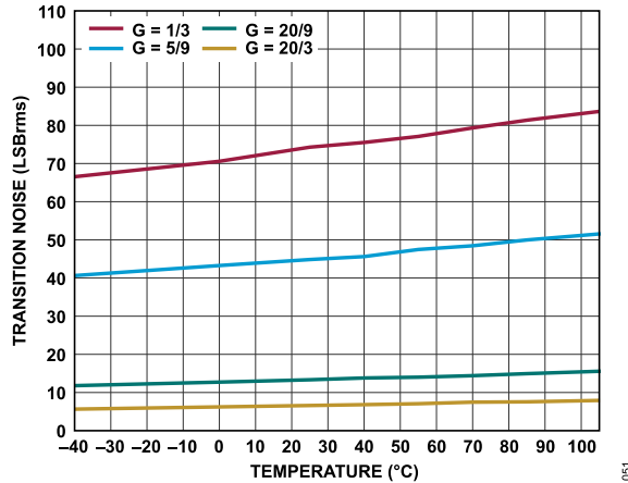
Figure 51. Transition Noise vs. Temperature, REFIN = 5 V
