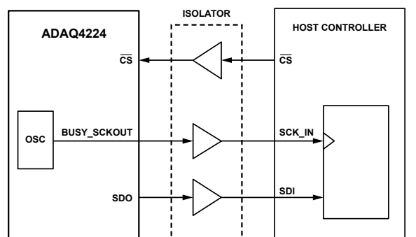
Figure 109. Host Clock Mode Signal Path Example
