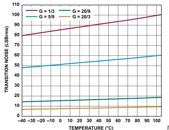
Figure 54. Transition Noise vs. Temperature, REFIN = 4.096 V
