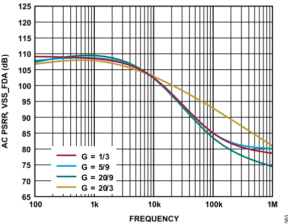
Figure 84. AC PSRR vs. Frequency, VSSH
