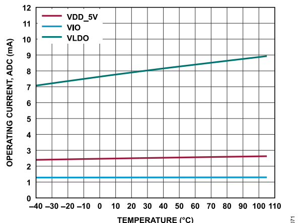
Figure 71. Operating Current ADC vs. Temperature
