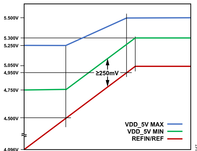
Figure 103. VDD_5V Minimum and Maximum Values for REFIN
