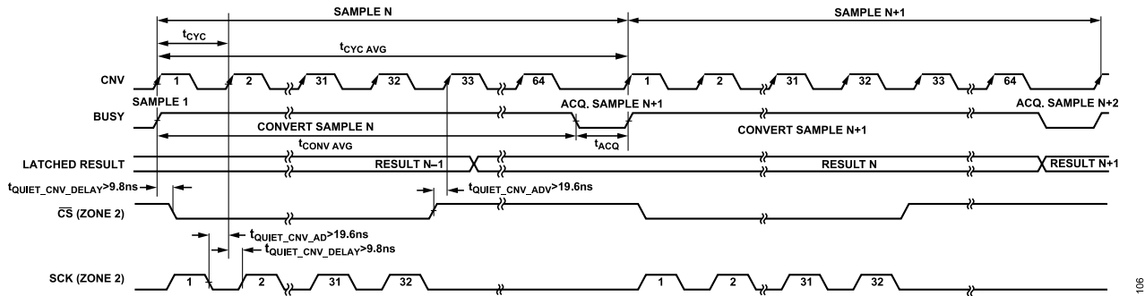
Figure 113. Example of Zone 2 in Averaging Mode (1 Bit per Sample)
