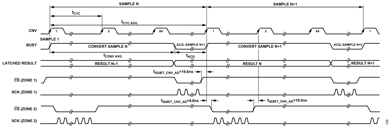
Figure 112. Example of Different Zones in Averaging Mode (64 Samples Averaged)
