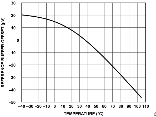
Figure 67. Reference Buffer Offset vs. Temperature
