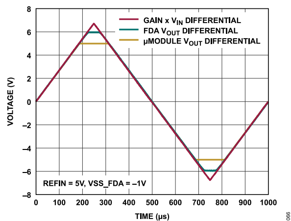
Figure 85. Output Overdrive Recovery, I_N = 1 \text{ kHz}
