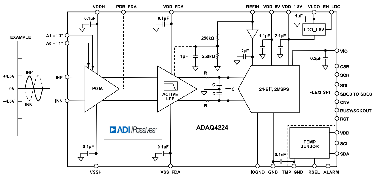
Figure 92. Differential Input Configuration with G = 5/9 \text{ V/V}
