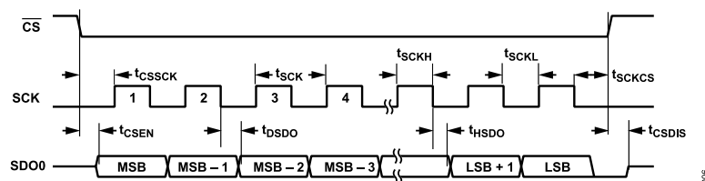
Figure 6. SPI Clocking Mode 1-Lane SDR Timing
