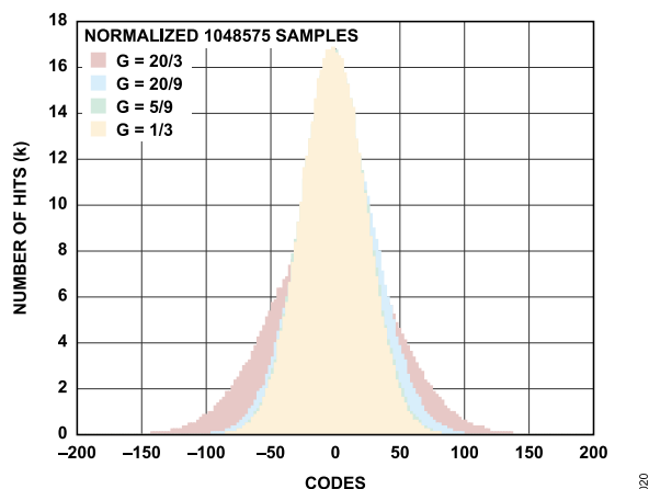
Figure 20. Code Histogram for Shorted Inputs, REFIN = 5\text{ V}
