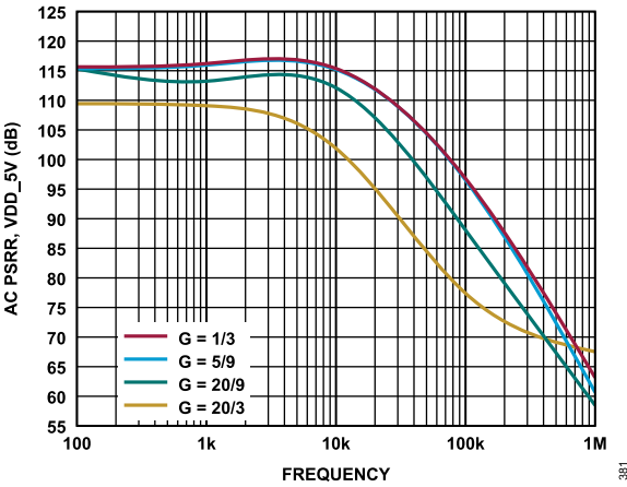
Figure 82. AC PSRR vs. Frequency, VDD_5V
