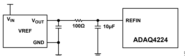
Figure 99. Reference with Noise Filter
