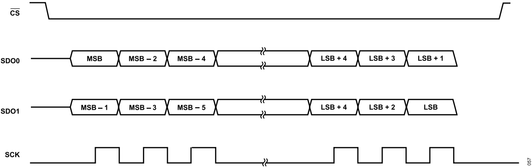
Figure 115. 2-Lane Mode, SDR Timing Diagram
