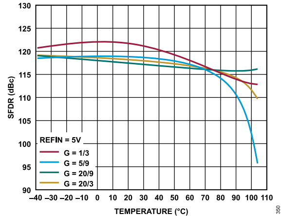
Figure 50. SFDR vs. Temperature, f_{IN} = 1 kHz, REFIN = 5 V
