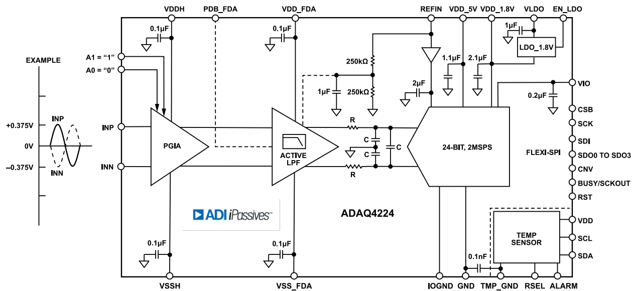
Figure 94. Differential Input Configuration with G = 20/3 V/V
