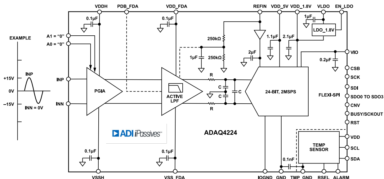
Figure 95. Single-Ended Input Configuration with G = 1/3 V/V
