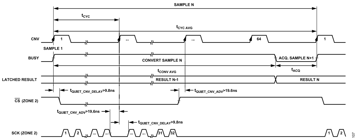
Figure 114. Example of Zone 2 in Averaging Mode (N Bits per Cycle)
