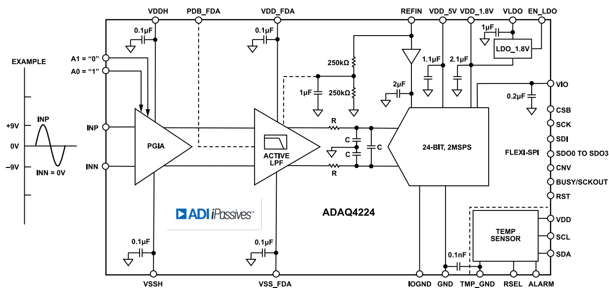
Figure 96. Single-Ended Input Configuration with G = 5/9 V/V
