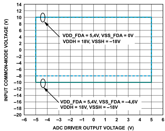
Figure 78. Input Common-Mode Voltage vs. ADC Driver Output Voltage, All Gains
