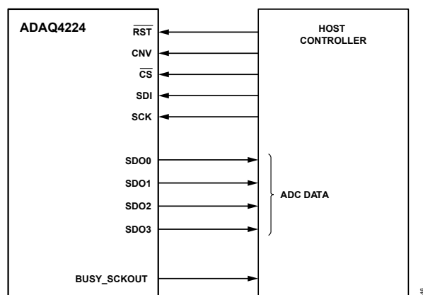
Figure 104. ADAQ4224 Multilane SPI
