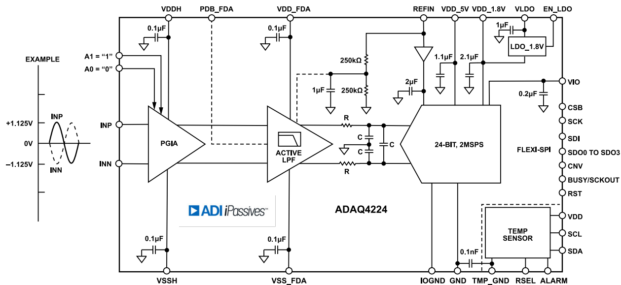
Figure 93. Differential Input Configuration with G = 20/9 V/V
