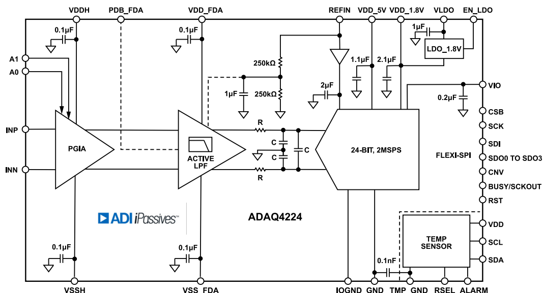
Figure 86. ADAQ4224 Functional Block Diagram
