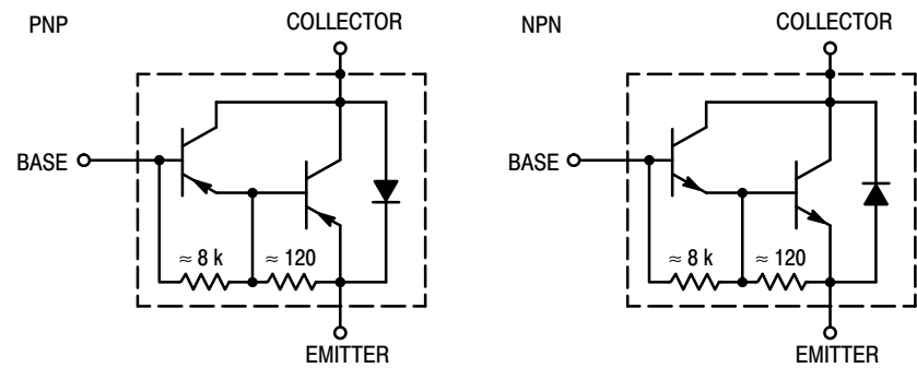
Figure 13. Darlington Schematic
