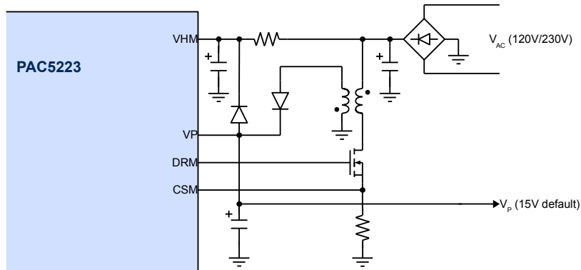
Figure 10-4. Flyback Mode
