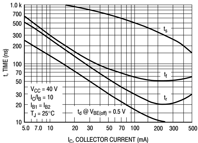
Figure 3. Switching Time
