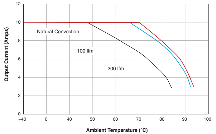
LSM-5/10-D12 Maximum Output Current vs. Ambient Temperature (SMT mount, air flow direction from pin 2 to pin 1)
