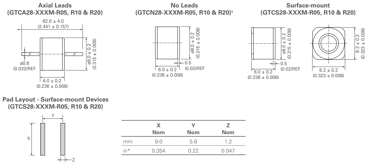
Figure G6 — Two Electrode 8mm Product Dimensions
