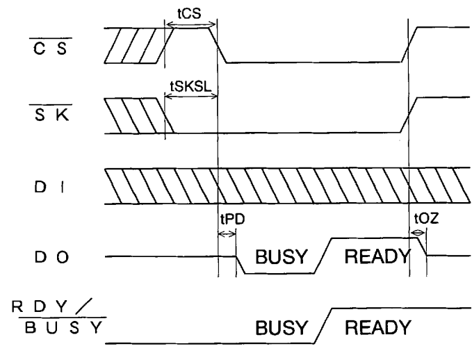
Ready / \overline{BUSY} Signal Output ( DO pin )
