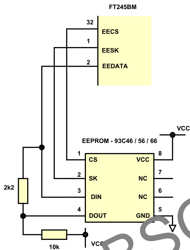
Figure 6 EEPROM Configuration
