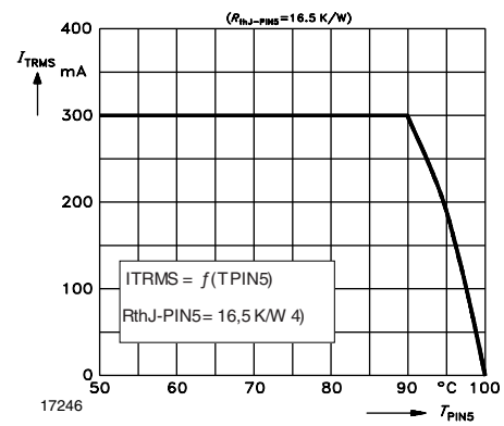
Fig. 8 - Current Reduction
