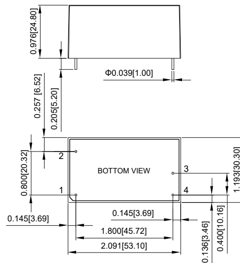
PIN CONNECTION
