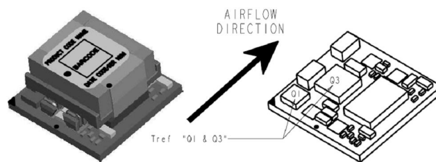
Preferred airflow direction and location of hot-spot of the module ( T_{ref} ).
