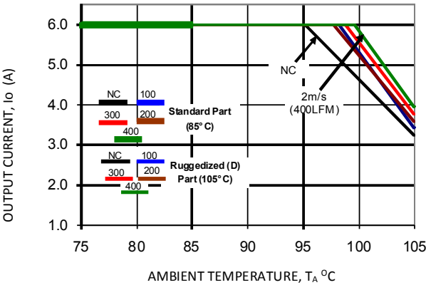
Vo=1.8V
