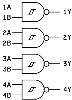
FIGURE 3. Logic diagram.
