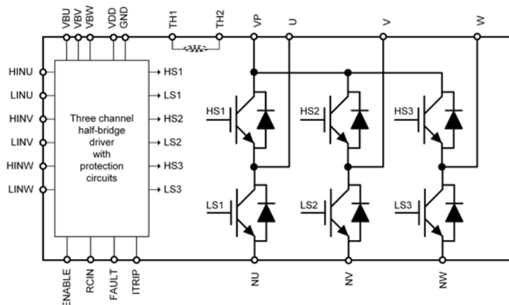
Figure 1. Functional Diagram
