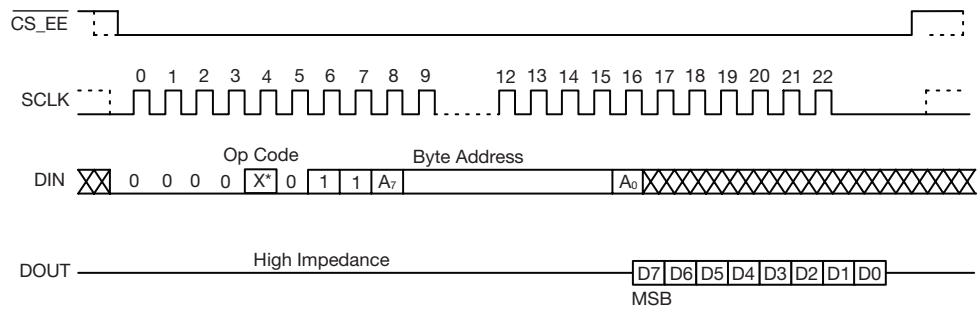
FIGURE 2-1. EEPROM COMMUNICATIONS
