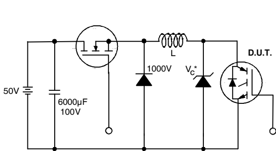
Fig. 19 - Clamped Inductive Load Test Circuit
