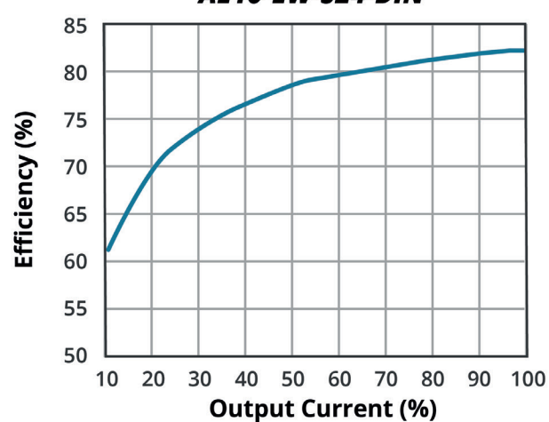
EFFICIENCY VS OUTPUT LOAD AE10-EW-S24-DIN
