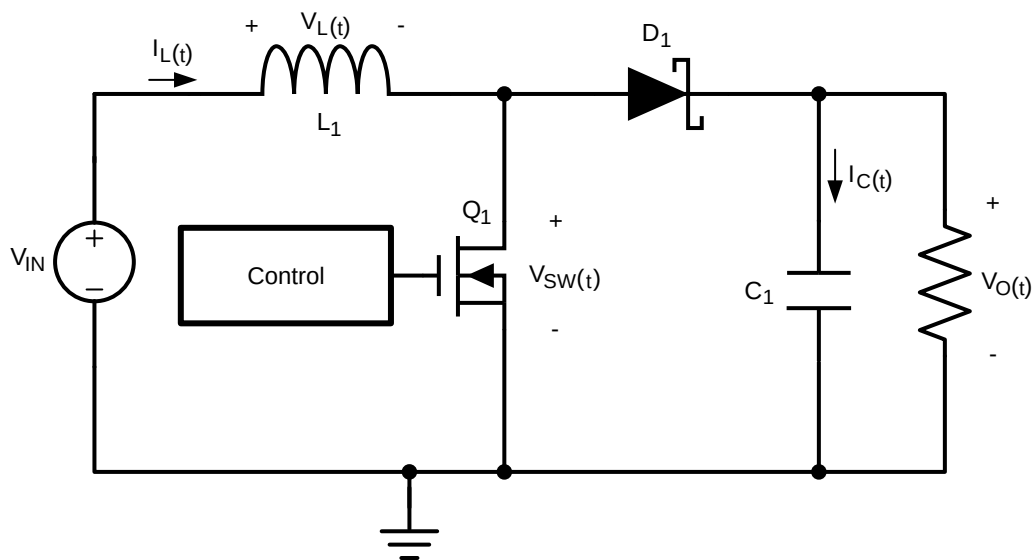
Figure 13. Simplified Schematic
